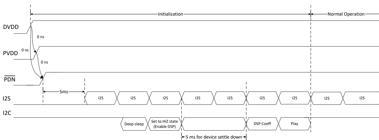
图 93. Start-up Sequence
