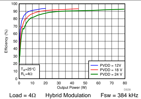
图 162. Efficiency vs Output Power
