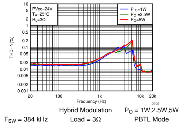
图 28. THD+N vs Frequency-PBTB
