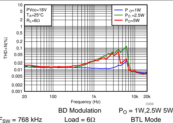
图 44. THD+N vs Frequency-BTL
