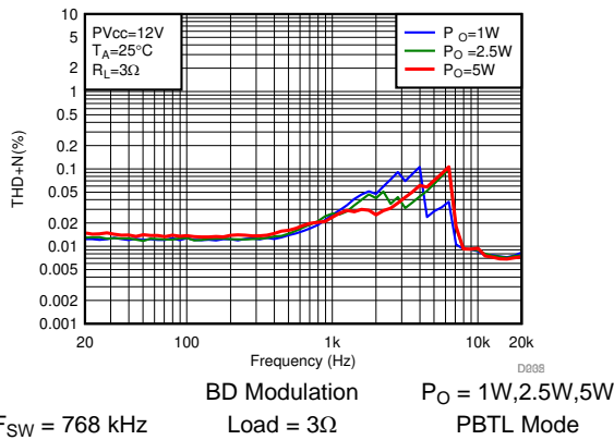
图 64. THD+N vs Frequency-PBTB
