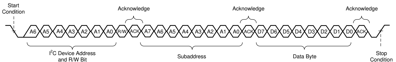
图 89. Random Write Transfer
