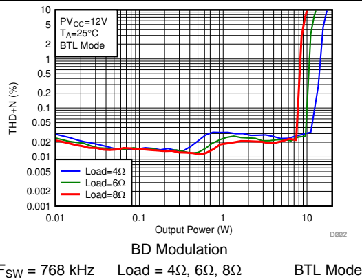
图 50. THD+N vs Output Power-BTL
