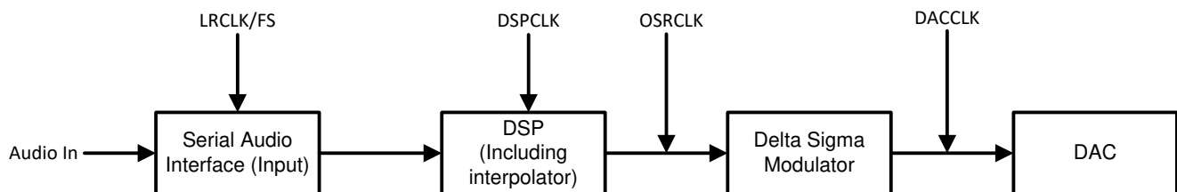
图 80. Audio Flow with Respective Clocks
