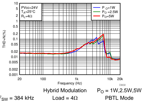
图 27. THD+N vs Frequency-PBTB
