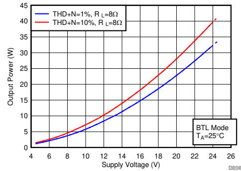
图 55. Output Power vs Supply Voltage
