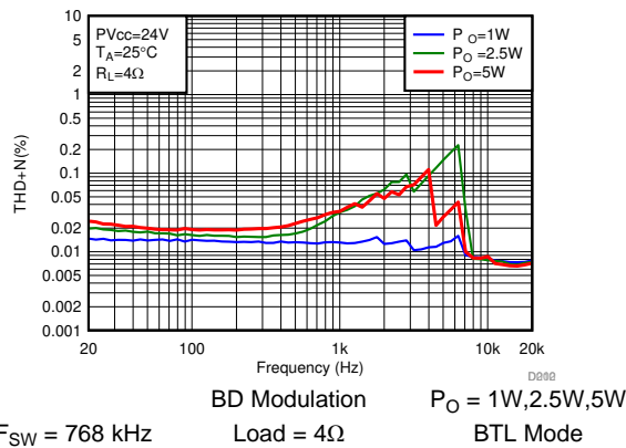
图 46. THD+N vs Frequency-BTL
