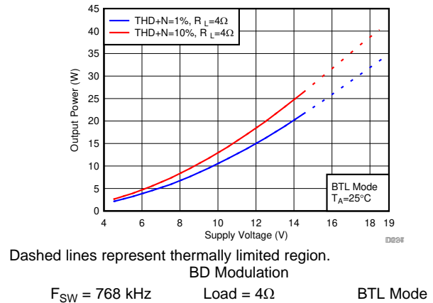
图 55. Output Power vs Supply Voltage
