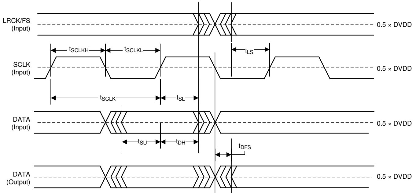
图 78. Serial Audio Port Timing in Slave Mode
