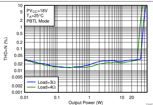
图 71. THD+N vs Output Power-PBTL
