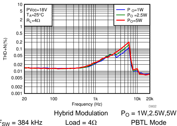
图 25. THD+N vs Frequency-PBTB
