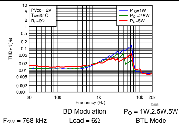
图 41. THD+N vs Frequency-BTL
