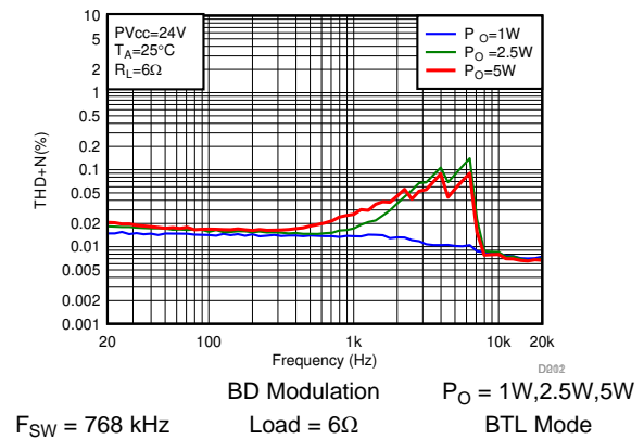
图 47. THD+N vs Frequency-BTL
