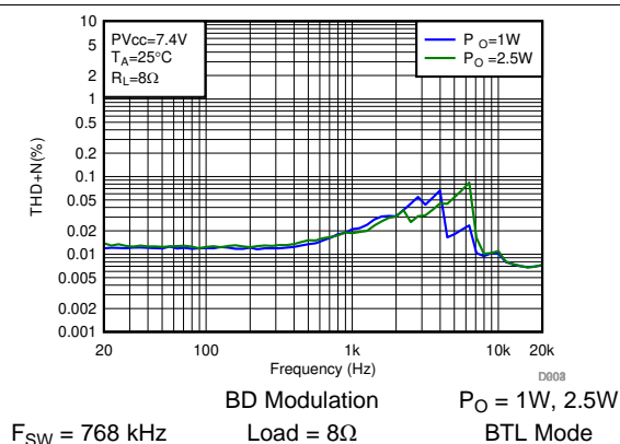
图 39. THD+N vs Frequency-BTL
