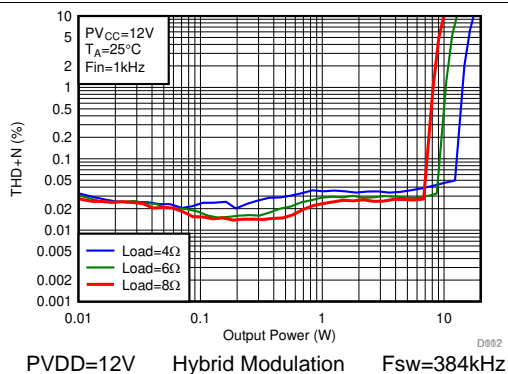
图 157. THD+N vs Power
