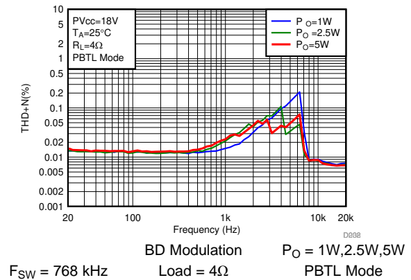
图 67. THD+N vs Frequency-PBTB
