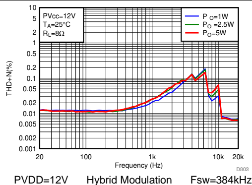
图 154. THD+N vs Frequency
