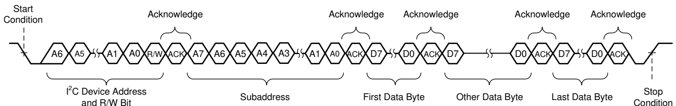
图 90. Sequential Write Transfer
