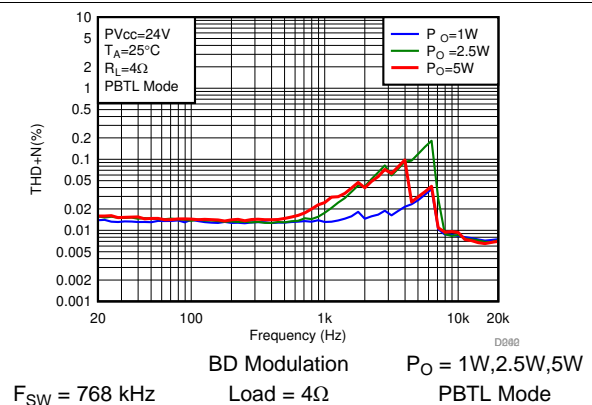
图 69. THD+N vs Frequency-PBTB
