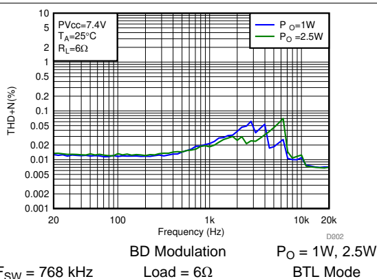
图 38. THD+N vs Frequency-BTL
