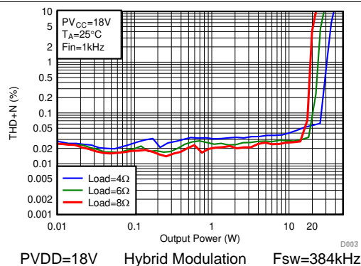
图 158. THD+N vs Power
