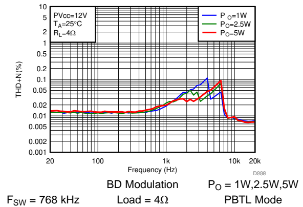
图 65. THD+N vs Frequency-PBTB
