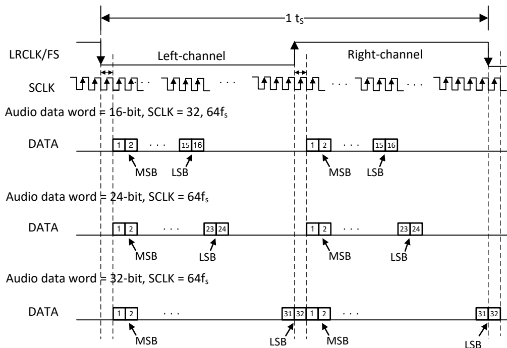
图 81. Left Justified Audio Data Format
