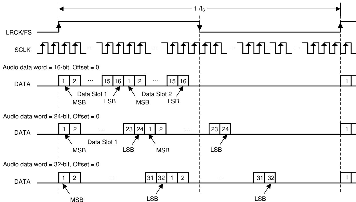
图 83. Right Justified Audio Data Format
