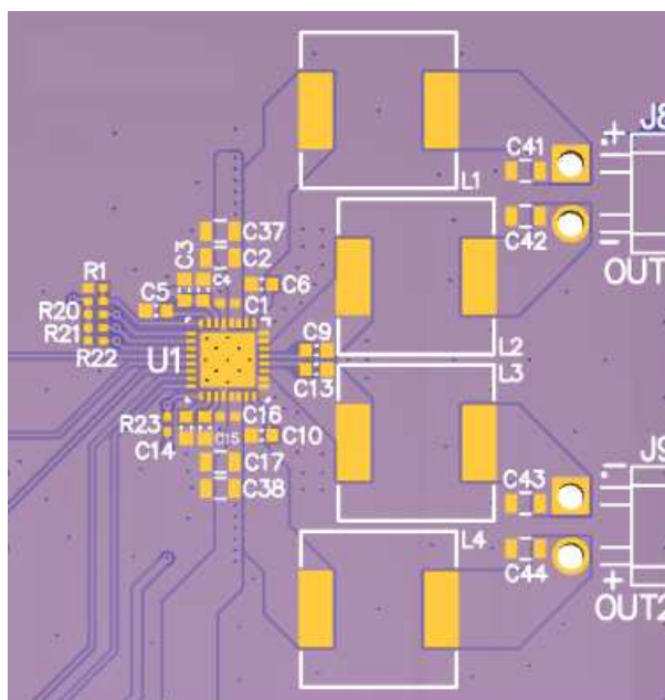
图 165. 2.0 (Stereo BTL) Top Copper View
