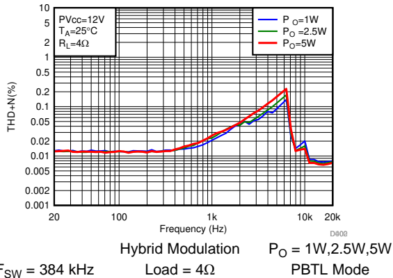
图 23. THD+N vs Frequency-PBTB
