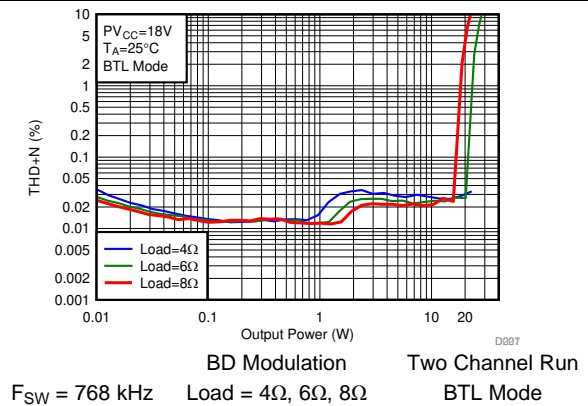
图 51. THD+N vs Output Power-BTL
