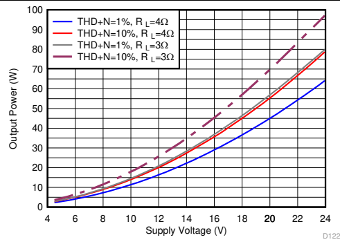
图 35. Output Power vs Supply Voltage
