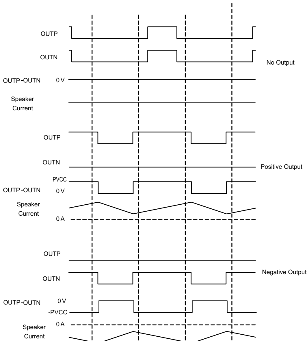
图 88. 1SPW Mode Modulation
