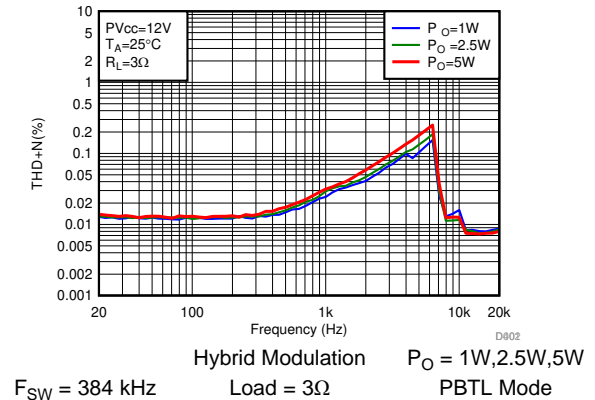
图 24. THD+N vs Frequency-PBTB
