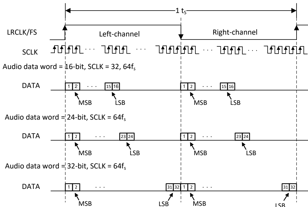
图 81. Left Justified Audio Data Format
