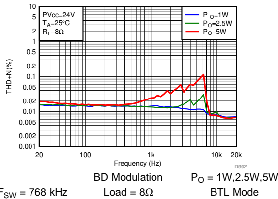
图 48. THD+N vs Frequency-BTL
