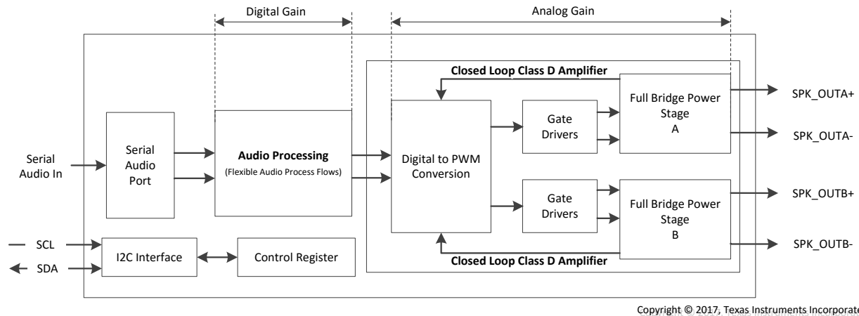
图 86. Speaker Amplifier Gain
