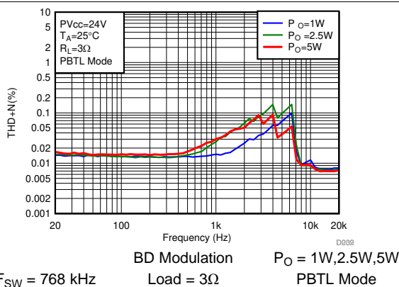
图 68. THD+N vs Frequency-PBTB
