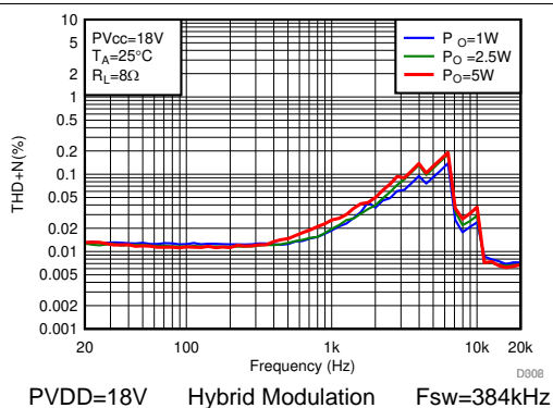
图 155. THD+N vs Frequency
