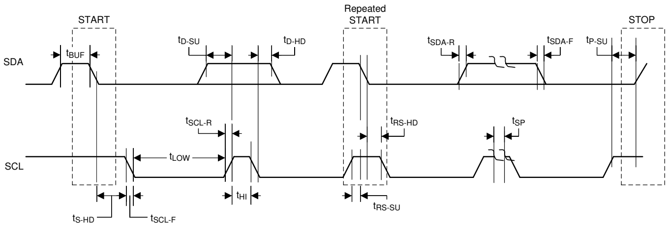
图 79. I²C Communication Port Timing Diagram
