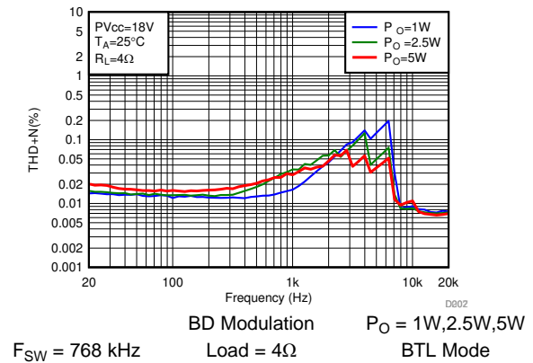
图 43. THD+N vs Frequency-BTL
