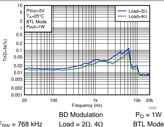
图 36. THD+N vs Frequency-BTL
