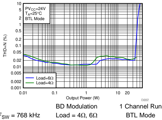
图 54. THD+N vs Output Power-BTL
