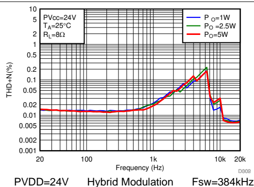
图 156. THD+N vs Frequency
