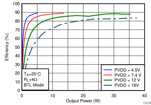
图 61. Efficiency vs Output Power
