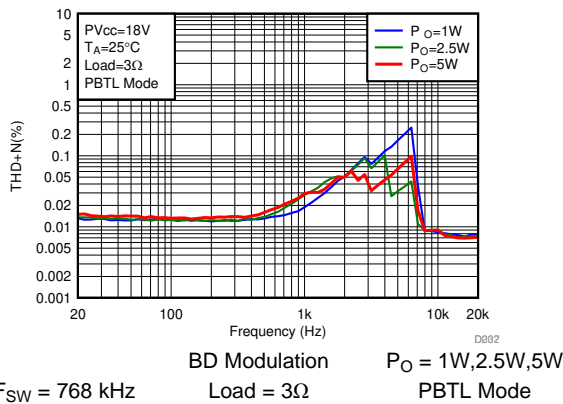
图 66. THD+N vs Frequency-PBTB
