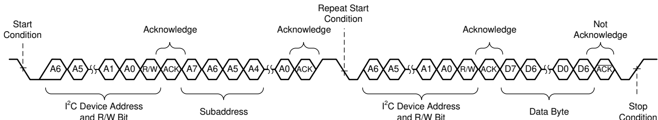
图 91. Random Read Transfer
