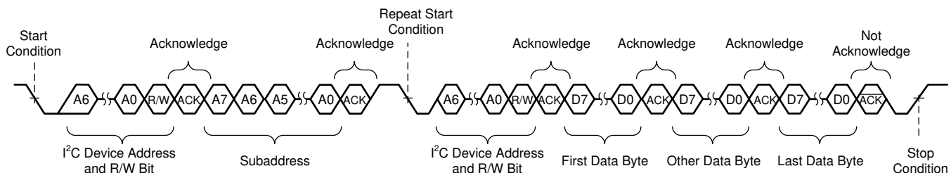
图 92. Sequential Read Transfer
