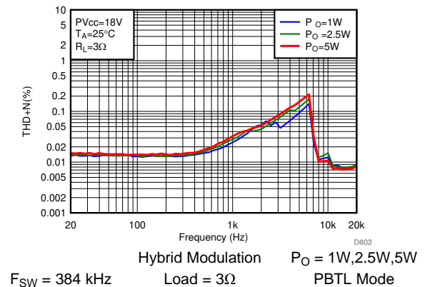
图 26. THD+N vs Frequency-PBTB
