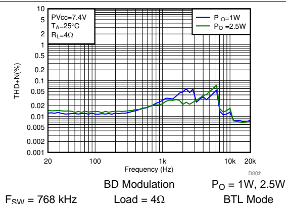
图 37. THD+N vs Frequency-BTL
