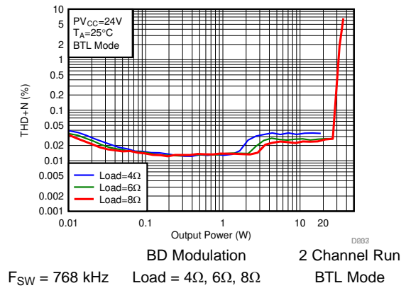
图 53. THD+N vs Output Power-BTL
