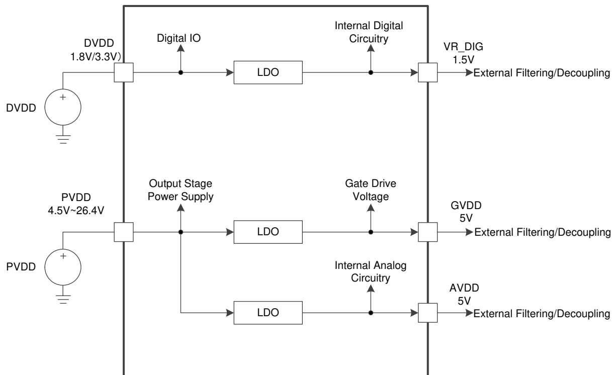
图 163. Power Supply Function Block Diagram
