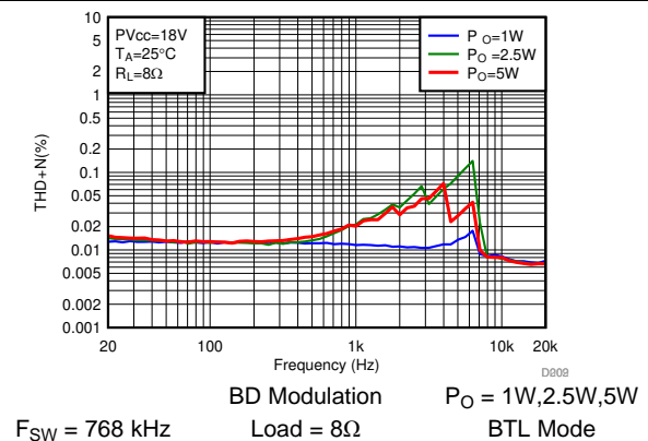
图 45. THD+N vs Frequency-BTL
