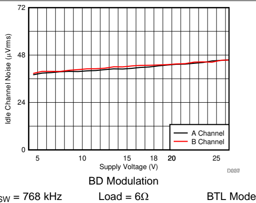
图 58. Idle Channel Noise vs Supply Voltage
