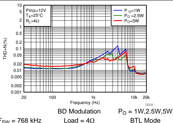
图 40. THD+N vs Frequency-BTL
