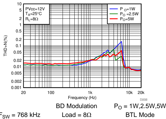
图 42. THD+N vs Frequency-BTL
