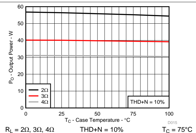
图 15. Output Power vs Case Temperature
