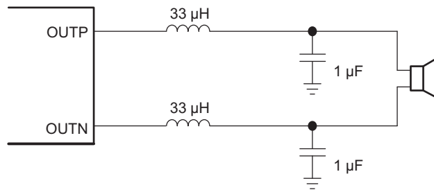
Figure 34. Typical LC Output Filter, Cutoff Frequency of 27 kHz
