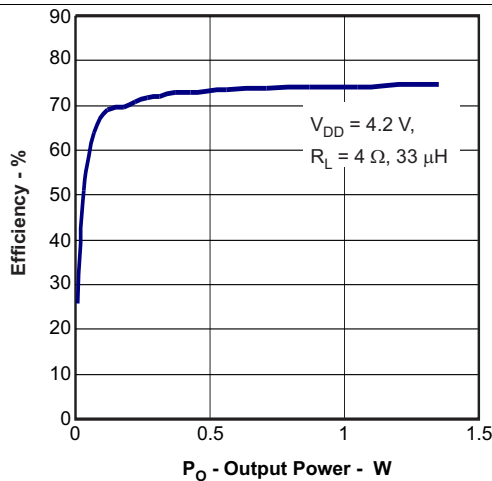
Figure 1. Efficiency vs Output Power
