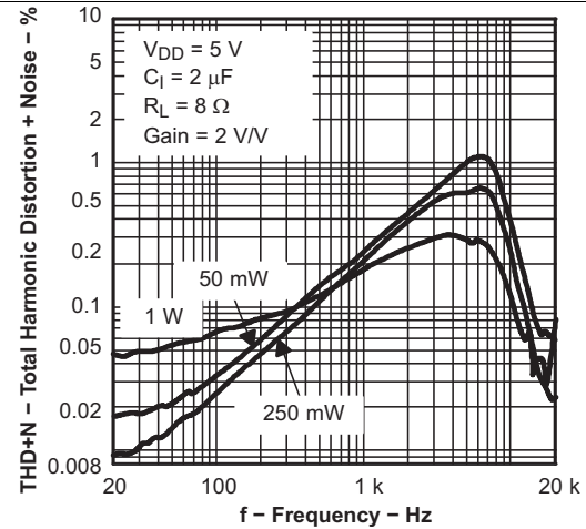
Figure 16. Total Harmonic Distortion + Noise vs Frequency
