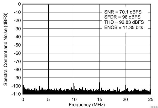
Figure 81. 5-MHz FFT, 50-MSPS Test for the Gain of 2 Interface in Figure 80
