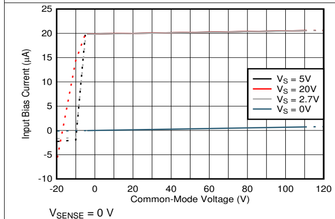
Figure 5. Input Bias Current vs Common-Mode Voltage
