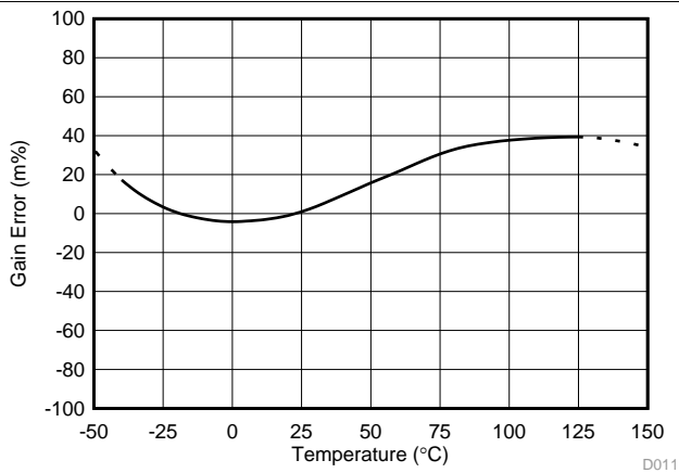
图 11. Bus Input Gain Error vs Temperature
