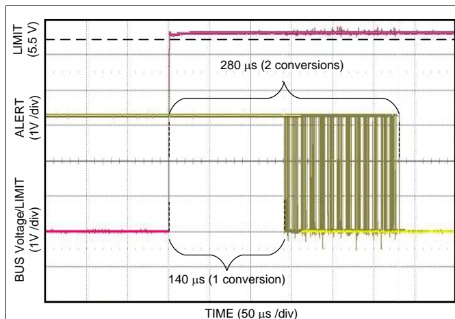
图 44. Alert Response ( t_{CT} = 140 \mu s)
