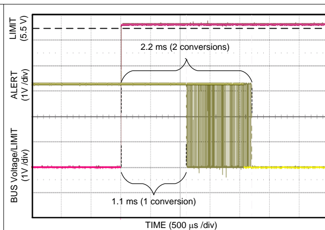
图 45. Alert Response ( t_{CT} = 1.1 ms)
