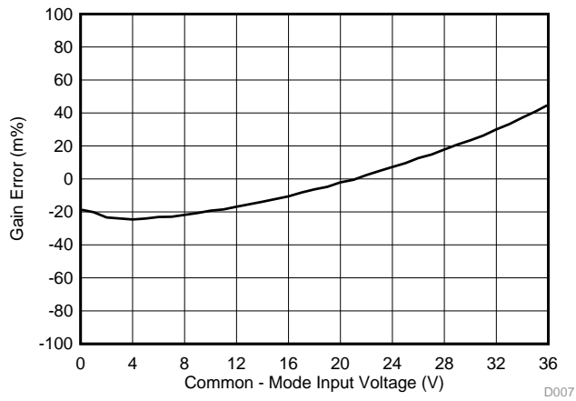
图 7. Shunt Input Gain Error vs Common-Mode Voltage
