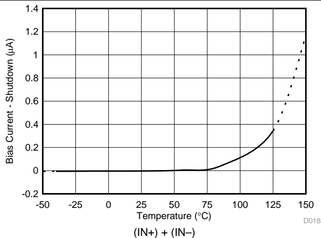
图 18. Input Bias Shutdown Current vs Temperature
