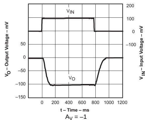
图 30. Small-Signal Step Response
