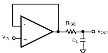
图 31. Resistive Isolation of Capacitive Load
