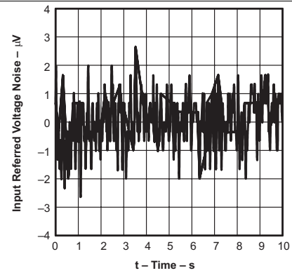
图 26. Voltage Noise Over a 10-Second Period
