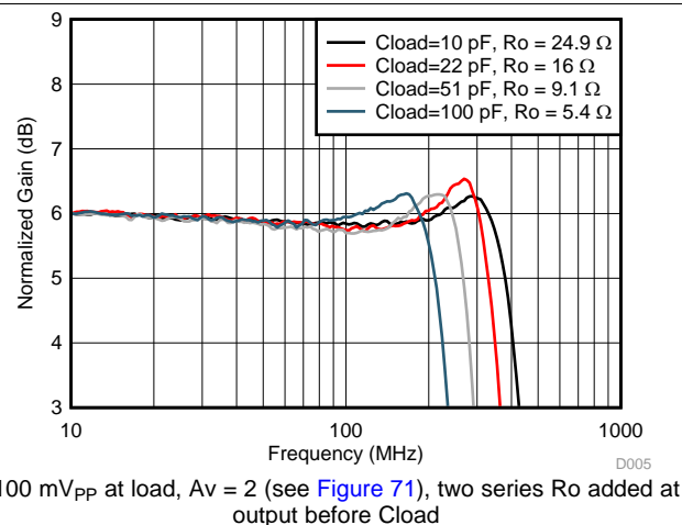
Figure 5. Small Signal Frequency response vs Cload
