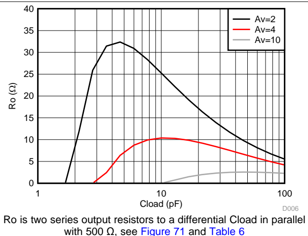
Figure 6. Recommended Ro vs Cload
