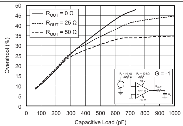
Figure 28. Small-Signal Overshoot versus Capacitive Load (100-mV Output Step)
