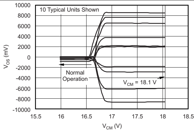
Figure 3. Offset Voltage vs Common-Mode Voltage: V_{\text{SUPPLY}} (\text{V}) = \pm 18 \text{ V} (Upper Stage)
