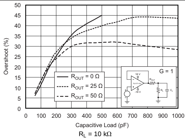
Figure 15. Noninverting Small-Signal Overshoot vs Capacitive Load (100-mV Output Step)
