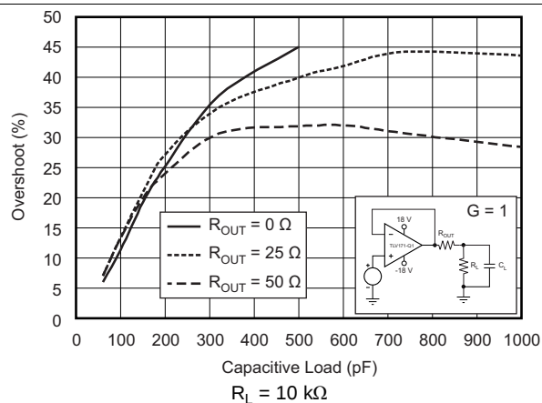
Figure 27. Small-Signal Overshoot versus Capacitive Load (100-mV Output Step)
