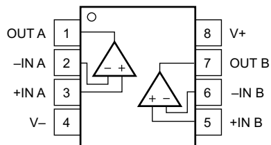
TLV2171-Q1 D or DGK Packages 8-Pin SOIC or VSSOP Top View
