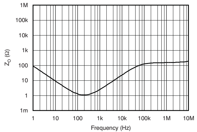
Figure 14. Open-Loop Output Impedance vs Frequency
