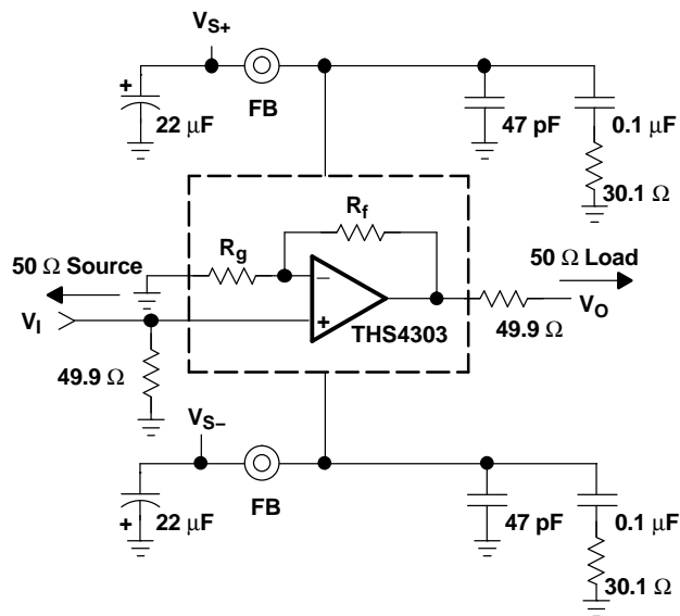
Figure 43. Wideband, Noninverting Gain Configuration
