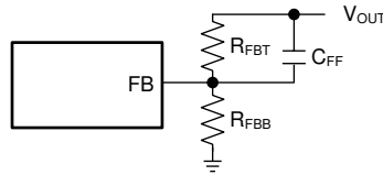
图 13. Feedforward Capacitor for Loop Compensation
