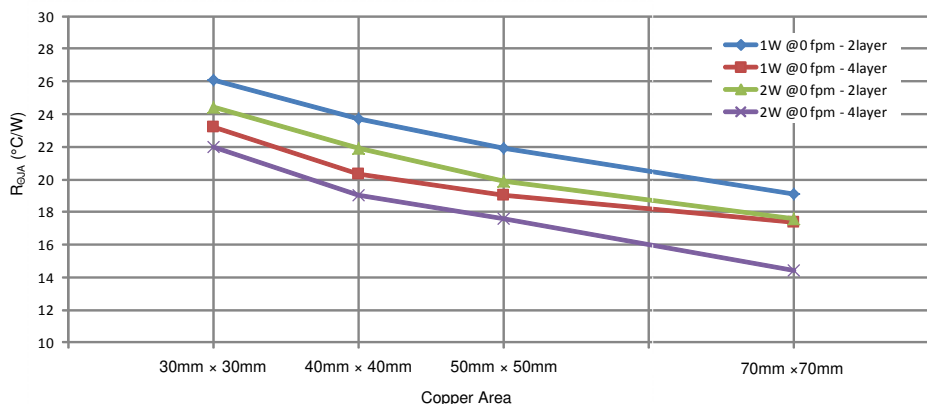
图 41. Measured R_{\theta JA} versus PCB Copper Area on a 2-Layer Board and a 4-Layer Board
