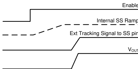
图 11. Tracking with Shorter Start-up Time than the Internal Ramp
