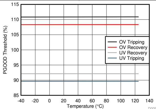
图 5. PGOOD Threshold
