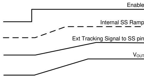
图 10. Tracking with Longer Start-up Time than the Internal Ramp
