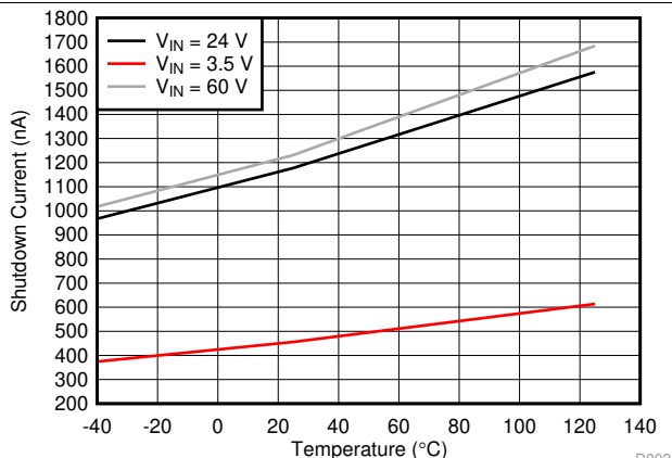
图 2. Shutdown Quiescent Current
