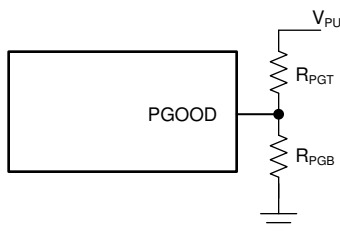
图 14. PGOOD Resistor Divider
