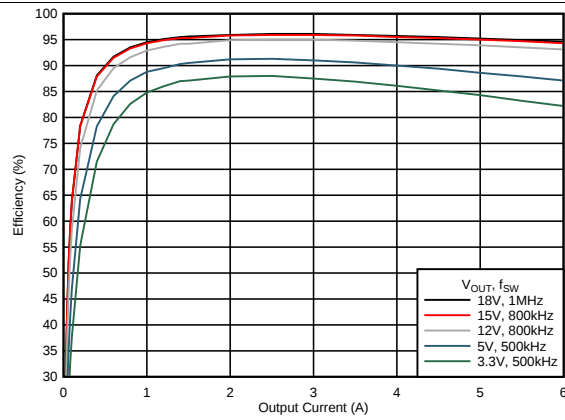
图 11. Efficiency vs Output Current
