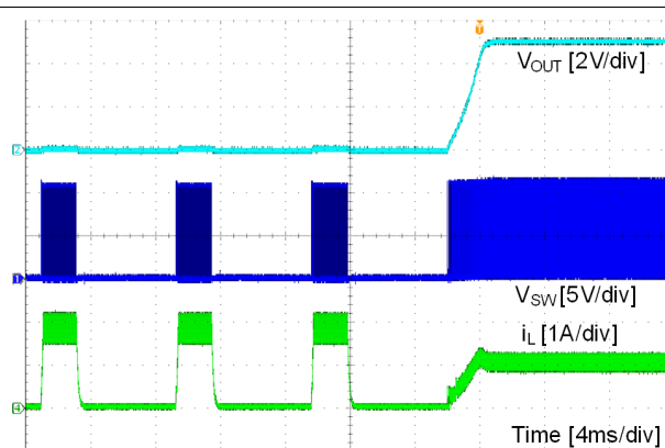
Figure 29. Short Recovery
