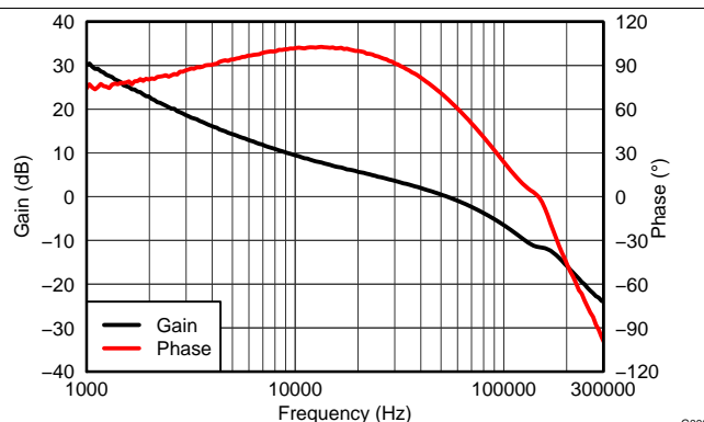
Figure 17. VOUT = 5 V, IOUT = 2 A, COUT1 = 44 \mu F ceramic, COUT2 = 56 \mu F electrolytic, fSW = 500 kHz
