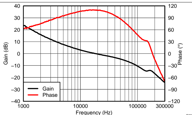
Figure 18. VOUT = 12 V, IOUT = 2 A, COUT1 = 44 \mu F ceramic, COUT2 = 56 \mu F electrolytic, fSW = 800 kHz
