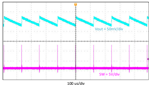
图 9-5. Output Voltage Ripple, 10 mA
