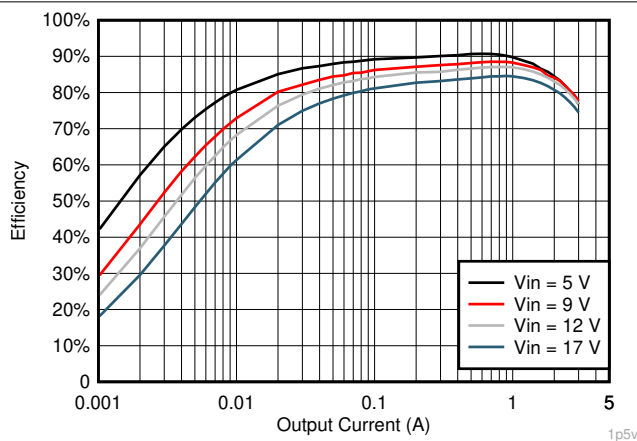
图 7-11. V_{OUT} = 1.5\text{ V} Efficiency, L = 1.5\text{ }\mu\text{H}
