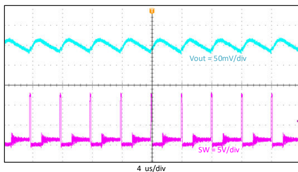
图 9-6. Output Voltage Ripple, I_{out} = 0.3\text{ A}
