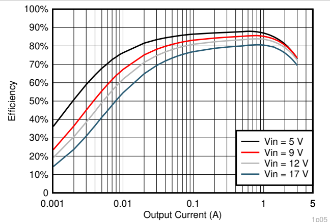
图 7-10. V_{OUT} = 1.05\text{ V} Efficiency, L = 1.2\text{ }\mu\text{H}
