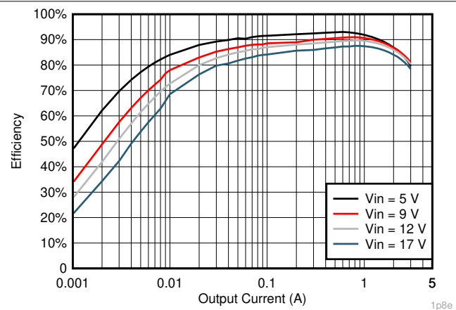
图 7-12. V_{OUT} = 1.8\text{ V} Efficiency, L = 2.2\text{ }\mu\text{H}
