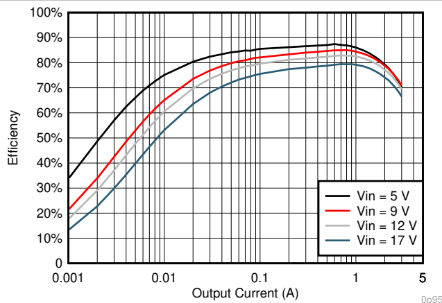
图 7-9. V_{OUT} = 0.95\text{ V} Efficiency, L = 1.2\text{ }\mu\text{H}
