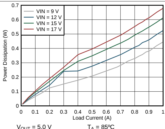
Figure 5. Power Dissipation
