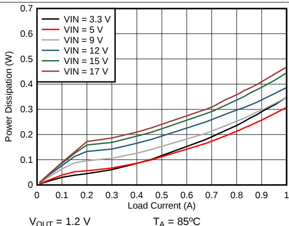
Figure 3. Power Dissipation
