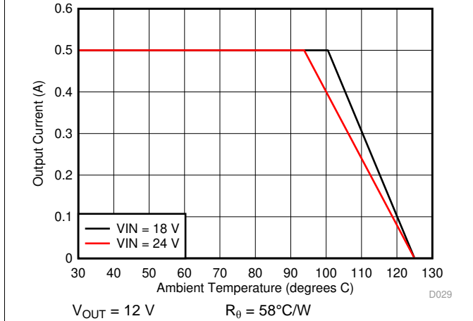
图 21. Ambient Temperature vs Output Current
