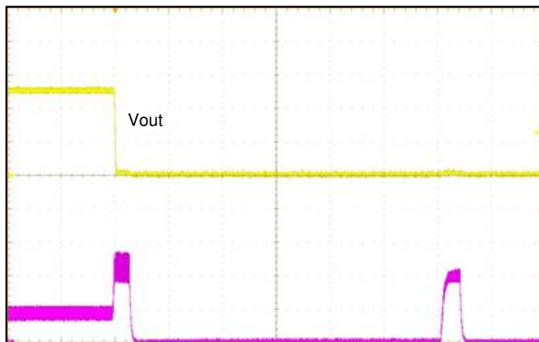
图 33. Hiccup Operation
