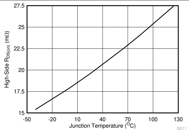
Figure 6-6. High-Side R_{DS(on)} vs Junction Temperature
