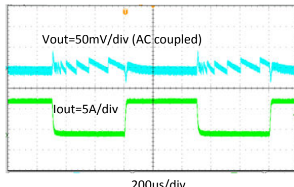
Figure 8-15. Transient Response, 0 A to 8 A
