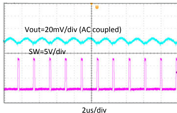
Figure 8-9. Output Voltage Ripple, I_{OUT} = 8 A
