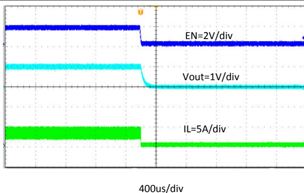
Figure 8-11. Shut-down Through EN, I_{OUT} = 4 A
