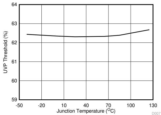
Figure 6-9. UVP Threshold vs Junction Temperature
