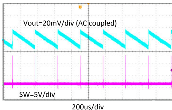
Figure 8-8. Output Voltage Ripple, I_{OUT} = 0.01 A
