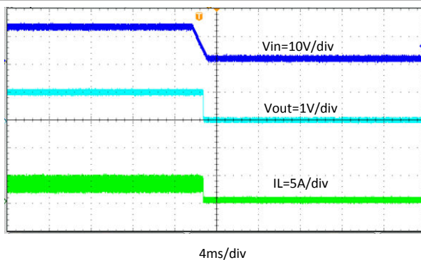
Figure 8-13. Start Up Relative to V_{IN} Falling, I_{OUT} = 4 A
