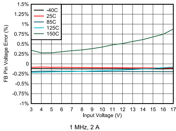
图 6-39. FB Pin Voltage Error vs Input Voltage
