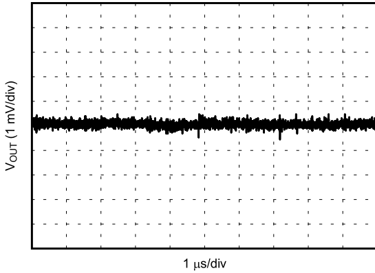
图 6-25. V_{OUT} Ripple After the Second L-C Filter
