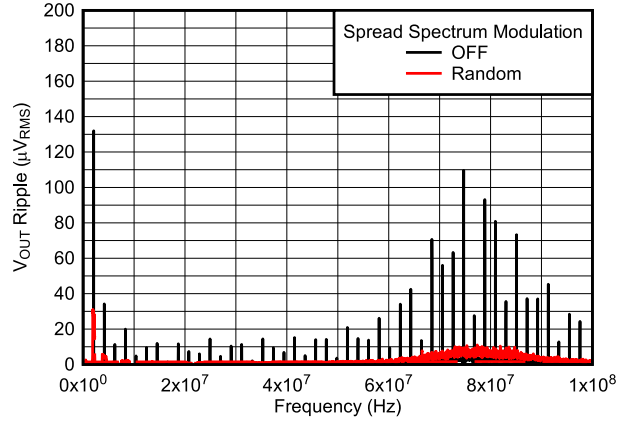
图 6-20. V_{OUT} Ripple FFT After the First L-C Filter ( V_{OUT-Mid} )
