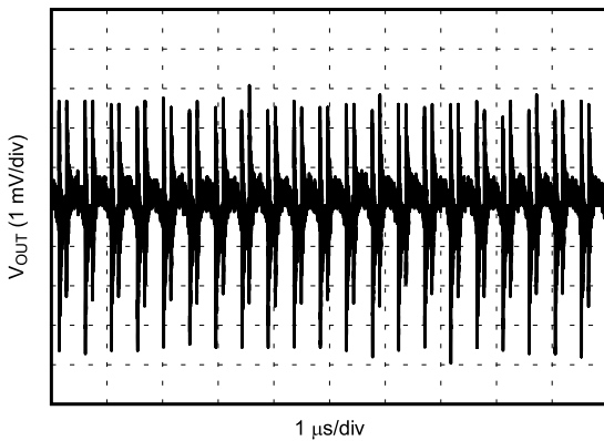
图 6-11. V_{OUT} Ripple After the First L-C Filter ( V_{OUT-Mid} )
