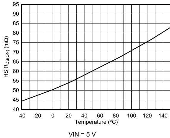
图 6-37. High-Side R_{DS(ON)} vs Junction Temperature
