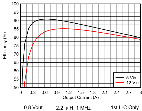
图 8-2. Efficiency vs Load Current
