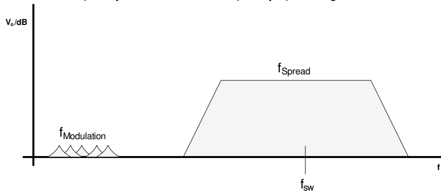
图 7-2. Randomized Spread Spectrum Modulation
