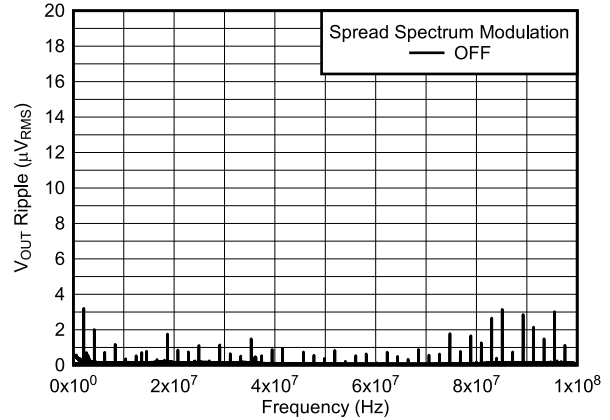
图 6-20. V_{OUT} Ripple FFT After the First L-C Filter ( V_{OUT-Mid} )
