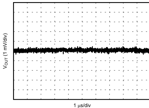
图 6-1. V_{OUT} Ripple After the First L-C Filter ( V_{OUT} -Mid)
