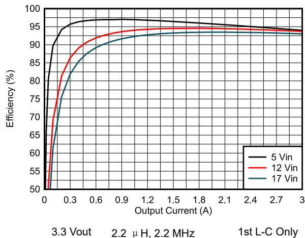
图 8-6. Efficiency vs Load Current
