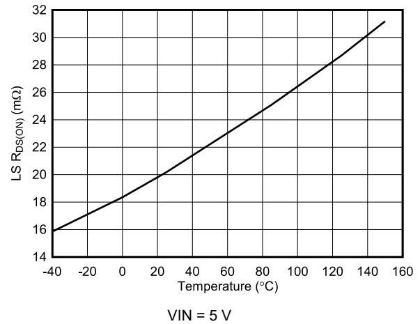
图 6-38. Low-Side R_{DS(ON)} vs Junction Temperature
