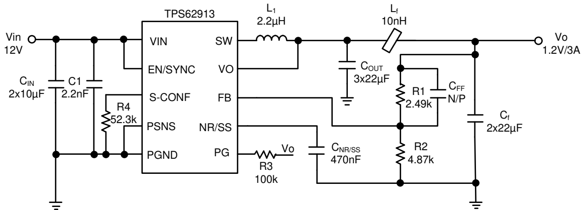
图 8-1. Typical Schematic
