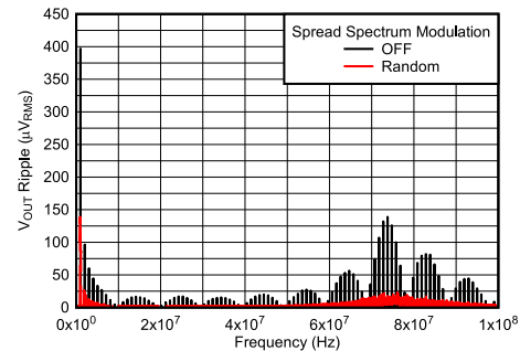
图 6-2. V_{OUT} Ripple FFT After the First L-C Filter ( V_{OUT} -Mid)
