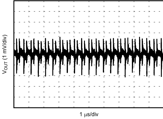
图 6-19. V_{OUT} Ripple After the First L-C Filter ( V_{OUT-Mid} )
