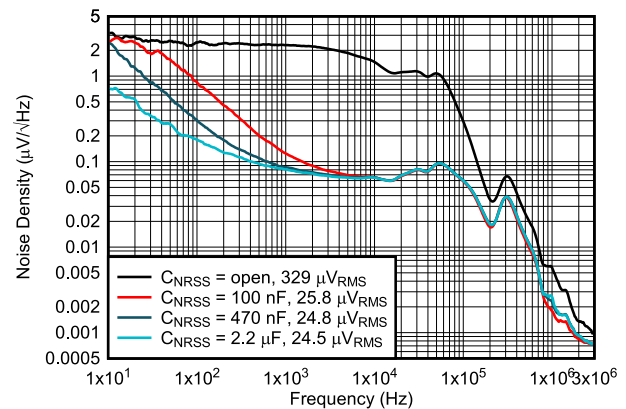
图 6-28. Output Noise Density vs Frequency
