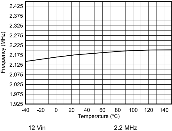
图 6-43. Oscillator Frequency vs Temperature
