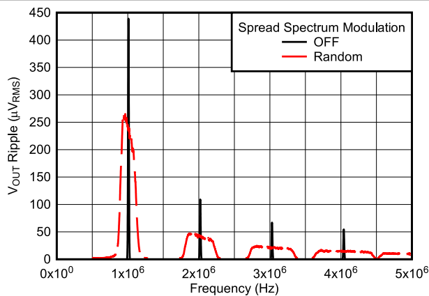
图 6-25. V_{OUT} Ripple After the Second L-C Filter
