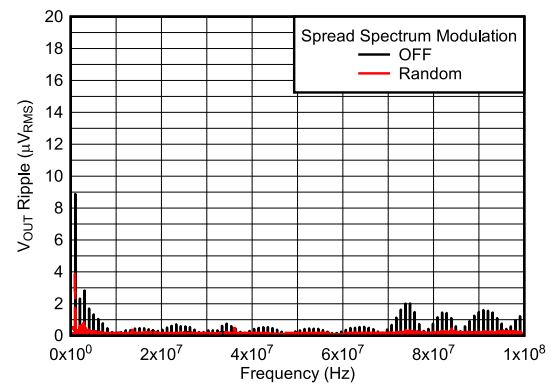
图 6-2. V_{OUT} Ripple FFT After the First L-C Filter ( V_{OUT} -Mid)
