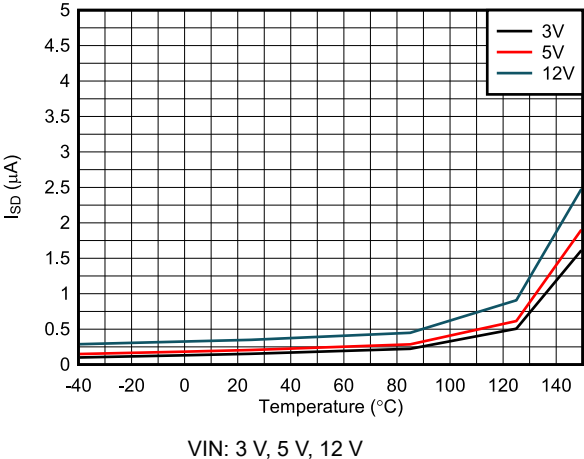
图 6-44. Shutdown Current vs Temperature
