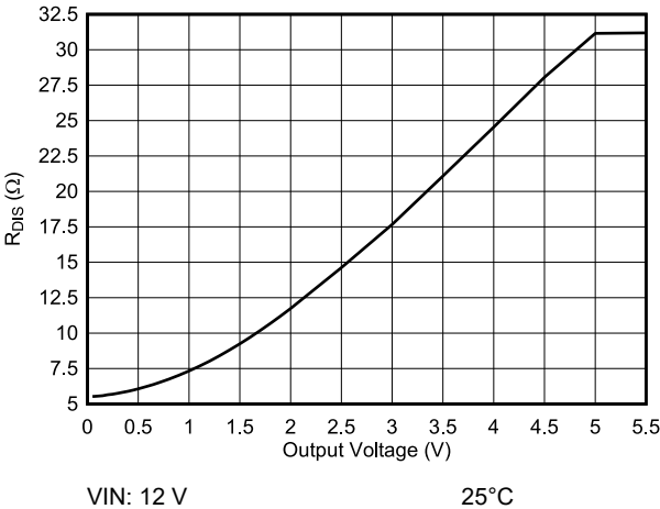
图 6-45. Output Discharge Resistance vs Output Voltage
