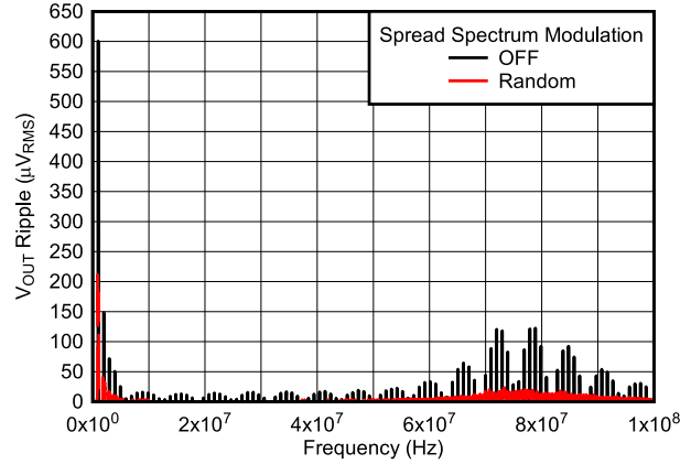
图 6-8. V_{OUT} Ripple FFT After the First L-C Filter ( V_{OUT-Mid} )
