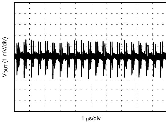
图 6-15. V_{OUT} Ripple After the First L-C Filter ( V_{OUT-Mid} )
