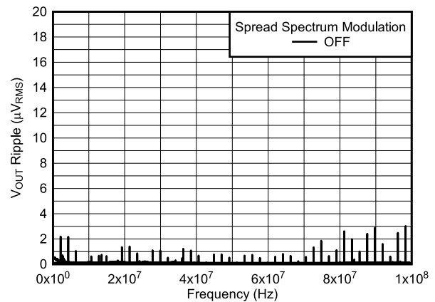
图 6-16. V_{OUT} Ripple FFT After the First L-C Filter ( V_{OUT-Mid} )
