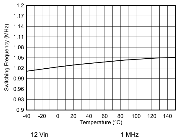
图 6-42. Oscillator Frequency vs Temperature
