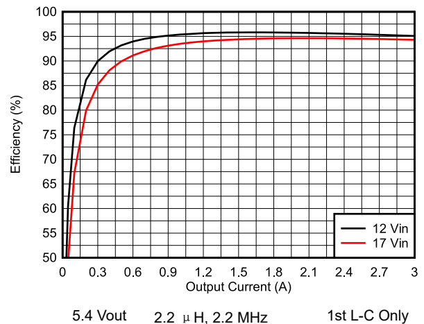
图 8-7. Efficiency vs Load Current
