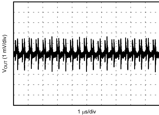
图 6-23. V_{OUT} Ripple After the First L-C Filter ( V_{OUT-Mid} )
