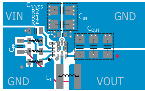
图 10-1. Recommended Layout for Single L-C Filter
