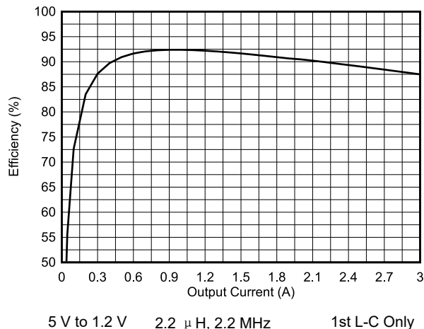
图 8-8. Efficiency vs Load Current
