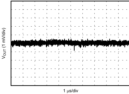
图 6-13. V_{OUT} Ripple After the Second L-C Filter
