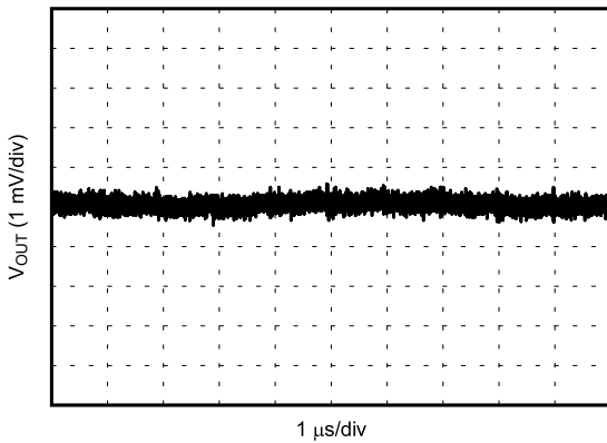
图 6-7. V_{OUT} Ripple After the First L-C Filter ( V_{OUT-Mid} )
