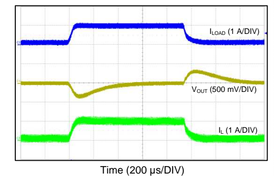
Figure 79. Output Voltage Regulation
