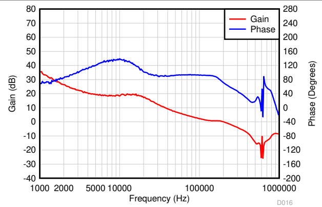
图 6-20. Frequency Response, 20 A Load
