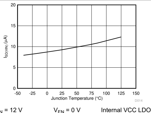
图 6-8. I_{SD(VIN)} vs Junction Temperature
