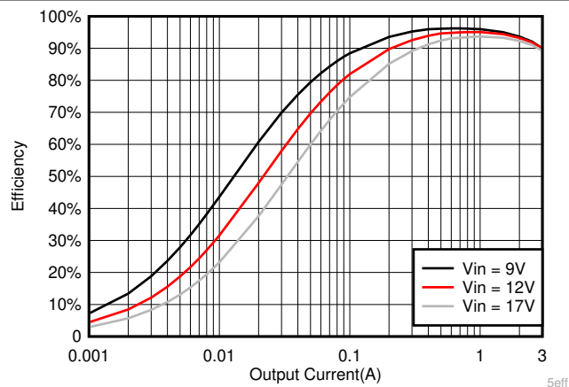
图 7-14. V_{OUT} = 5\text{-V} Efficiency, L = 4.7\text{ }\mu\text{H}
