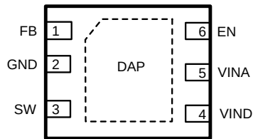
Figure 1. 6-Pin WSON
