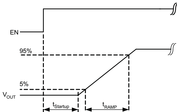
Figure 7. Soft-Start
