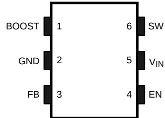
DDC Package 6-Pin SOT-23-THIN Top View
