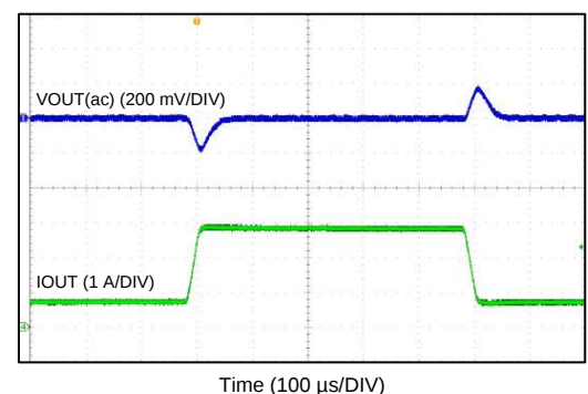
Figure 26. DCM Mode
