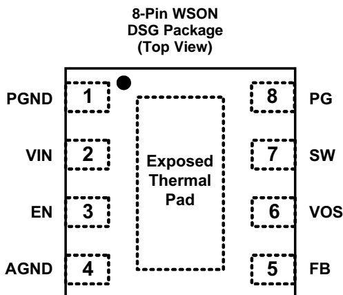
Pin Functions
