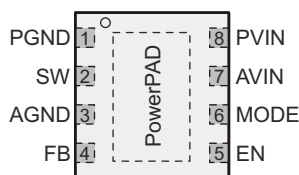
图 6-1. DSG Package 8-Pin WSON Top View
