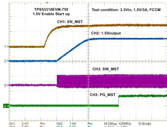
Figure 24. 1.5-V Turnon Waveform (3.3 VIN, 1.5 V/3 A)
