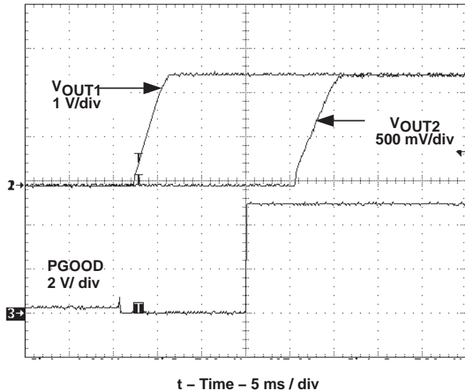
Figure 19. Offset Startup
