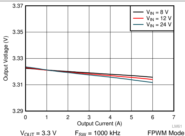
图 49. LM61460 Load and Line Regulation
