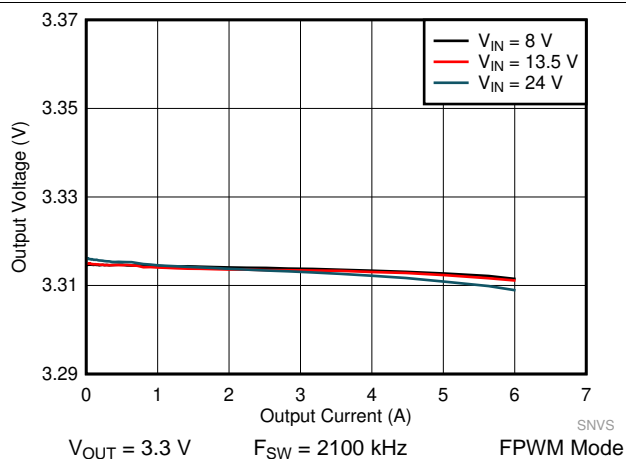
图 51. LM61460 Load and Line Regulation
