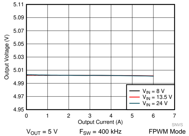
图 53. LM61460 Load and Line Regulation
