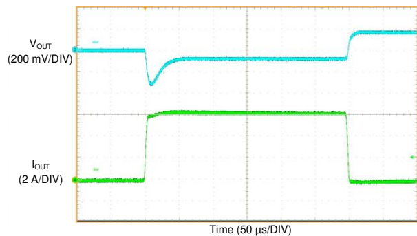
V_{OUT} = 5\text{ V} F_{SW} = 2100\text{ kHz} AUTO Mode I_{OUT} = 0\text{ A to }6\text{ A to }0\text{ A} V_{IN} = 13.5\text{ V} T_R = T_F = 6\text{ μs}
