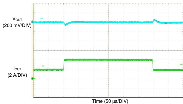
V_{OUT} = 3.3\text{ V} F_{SW} = 400\text{ kHz} AUTO Mode I_{OUT} = 2\text{ A to }4\text{ A to }2\text{ A} V_{IN} = 13.5\text{ V} T_R = T_F = 2\text{ μs}
