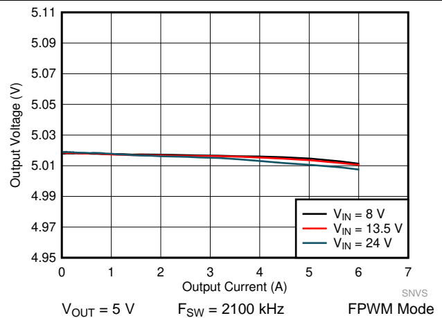
图 57. LM61460 Load and Line Regulation
