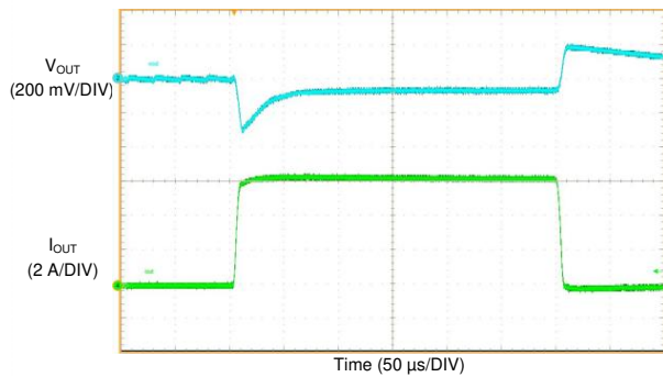
V_{OUT} = 5\text{ V} F_{SW} = 400\text{ kHz} AUTO Mode I_{OUT} = 50\text{ mA to }6\text{ A to }50\text{ mA} V_{IN} = 13.5\text{ V} T_R = T_F = 6\text{ μs}
