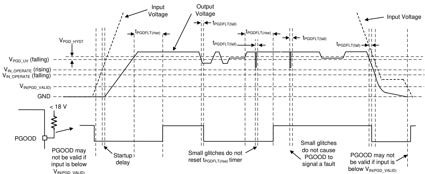
图 13. PGOOD Timing Diagram (Excludes OV Events)
