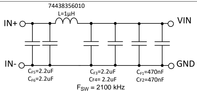
图 93. Recommended Input EMI Filter
