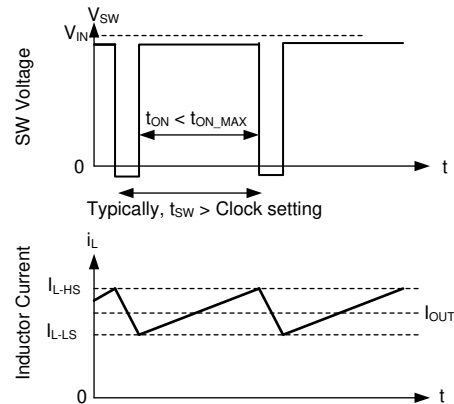
图 20. Current Limit Waveforms
