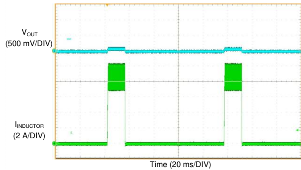
图 71. LM61460 Short Circuit Protection
