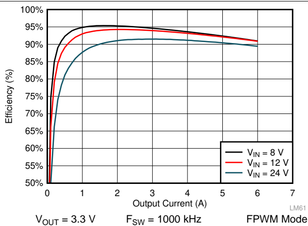
图 37. LM61460 Efficiency
