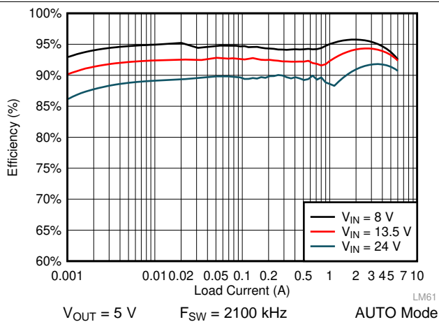
图 44. LM61460 Efficiency
