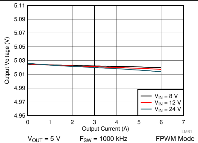
图 55. LM61460 Load and Line Regulation
