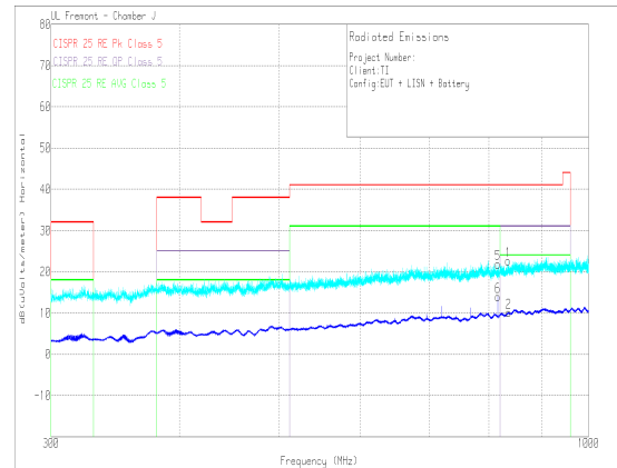
图 89. Radiated EMI Log Horizontal versus CISPR25 Limits
