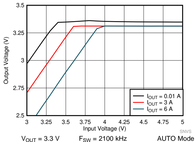
图 59. LM61460 Dropout Curve
