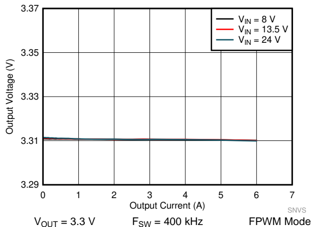
图 47. LM61460 Load and Line Regulation
