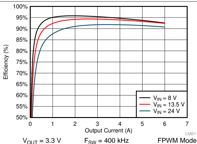
图 35. LM61460 Efficiency
