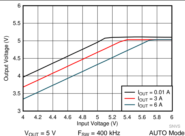
图 60. LM61460 Dropout Curve
