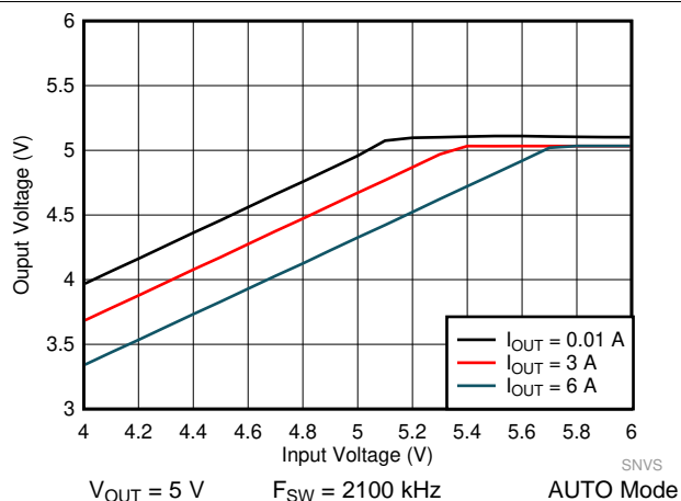
图 61. LM61460 Dropout Curve
