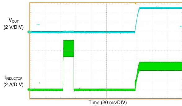
图 70. LM61460 Start-up with 3.25-A
