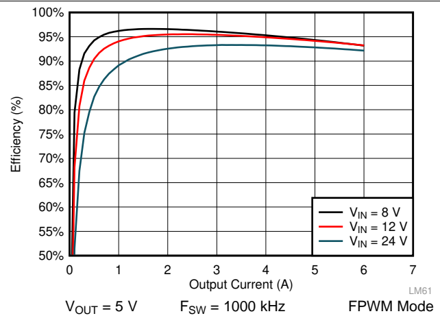
图 43. LM61460 Efficiency
