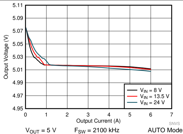
图 56. LM61460 Load and Line Regulation
