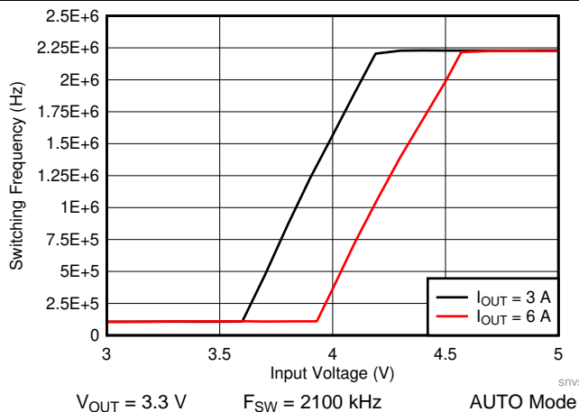
图 63. LM61460 Frequency Dropout Curve
