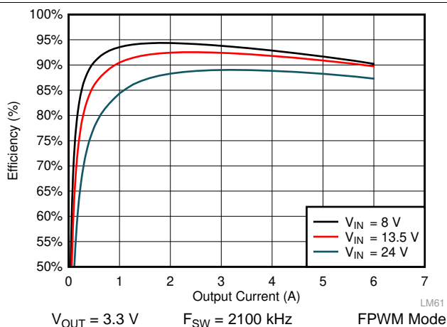
图 39. LM61460 Efficiency
