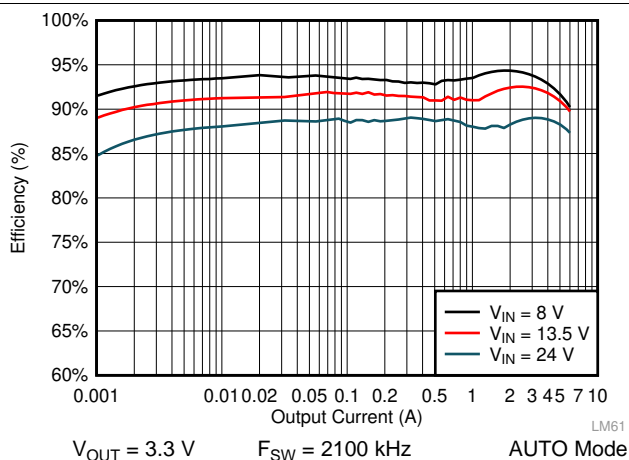
图 38. LM61460 Efficiency
