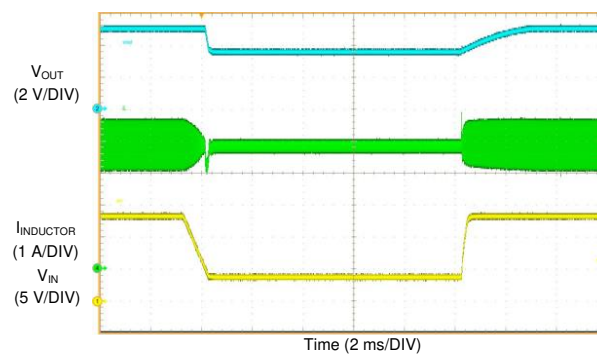
图 17. Recovery From Dropout ( V_{OUT} = 5\text{ V} , I_{OUT} = 4\text{ A} , V_{IN} = 13.5\text{ V} to 4\text{ V} to 13.5\text{ V} )
