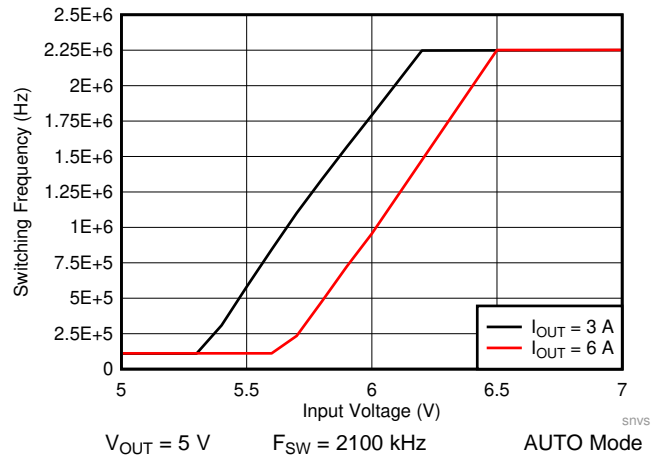
图 65. LM61460 Frequency Dropout Curve
