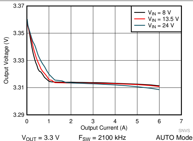
图 50. LM61460 Load and Line Regulation
