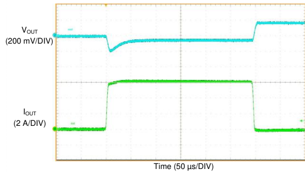
V_{OUT} = 3.3\text{ V} F_{SW} = 400\text{ kHz} AUTO Mode I_{OUT} = 0\text{ A to }6\text{ A to }0\text{ A} V_{IN} = 13.5\text{ V} T_R = T_F = 6\text{ μs}
