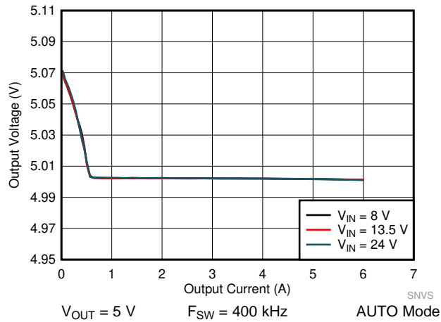
图 52. LM61460 Load and Line Regulation
