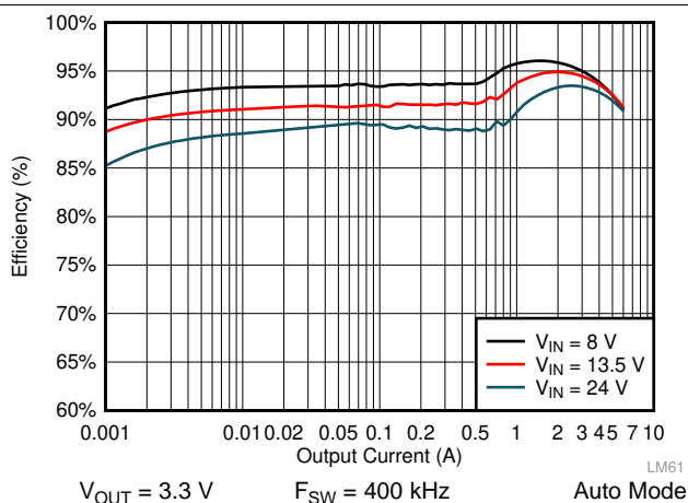
图 34. LM61460 Efficiency
