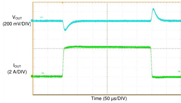
V_{OUT} = 5\text{ V} F_{SW} = 400\text{ kHz} FPWM Mode I_{OUT} = 0\text{ A to }6\text{ A to }0\text{ A} V_{IN} = 13.5\text{ V} T_R = T_F = 6\text{ μs}
