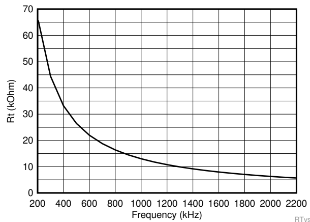
图 12. Setting Clock Frequency
