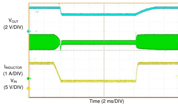
图 72. LM61460 Short Circuit Recovery
