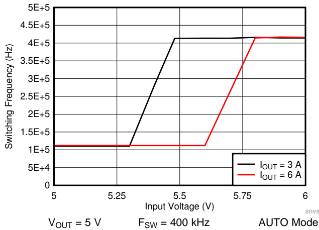
图 64. LM61460 Frequency Dropout Curve
