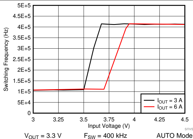
图 62. LM61460 Frequency Dropout
