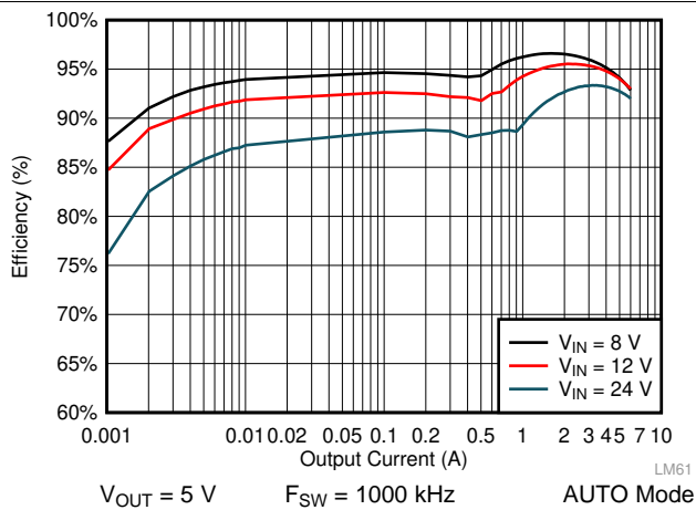
图 42. LM61460 Efficiency
