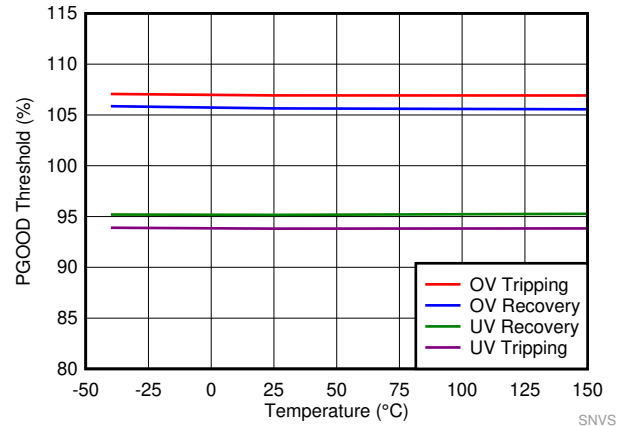
图 8. PGOOD Thresholds
