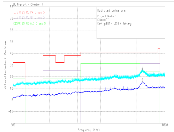
图 88. Radiated EMI Log Vertical versus CISPR25 Limits
