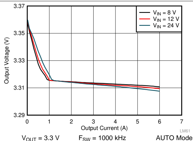
图 48. LM61460 Load and Line Regulation
