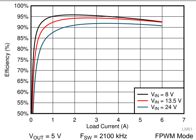
图 45. LM61460 Efficiency
