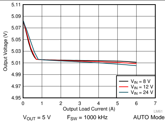
图 54. LM61460 Load and Line Regulation
