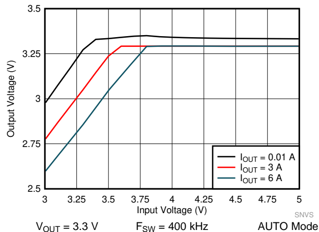
图 58. LM61460 Dropout Curve
