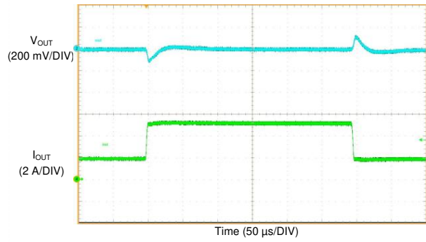
V_{OUT} = 5\text{ V} F_{SW} = 400\text{ kHz} AUTO Mode I_{OUT} = 2\text{ A to }5\text{ A to }2\text{ A} V_{IN} = 13.5\text{ V} T_R = T_F = 3\text{ μs}
