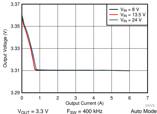
图 46. LM61460 Load and Line Regulation
