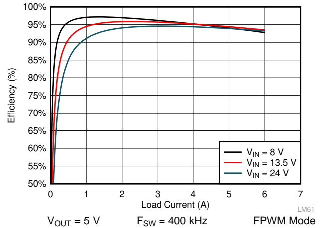
图 41. LM61460 Efficiency
