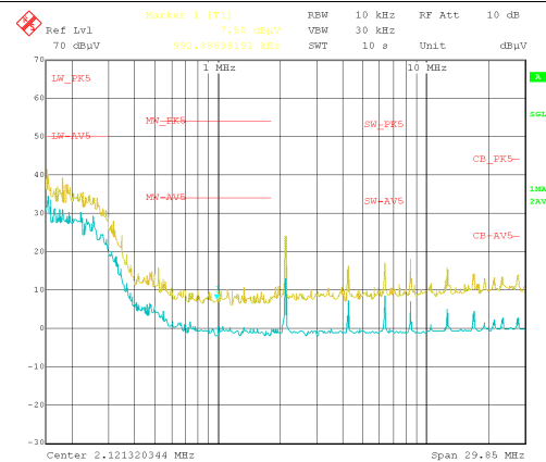
图 89. Radiated EMI Log Horizontal versus CISPR25 Limits
