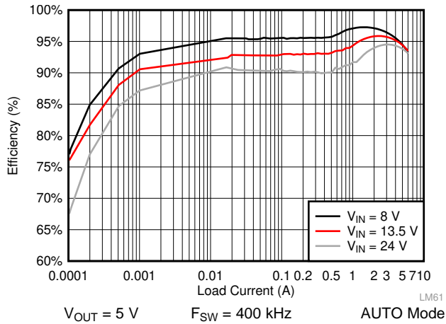
图 40. LM61460 Efficiency
