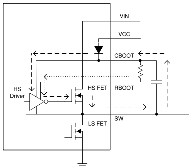
图 14. Simplified Circuit Showing How RBOOT Functions
