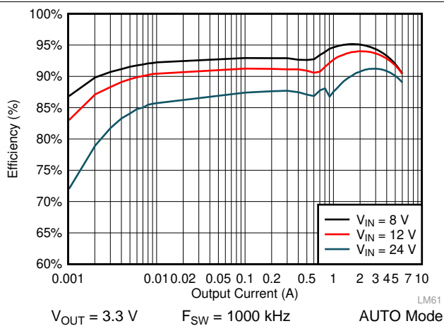
图 36. LM61460 Efficiency
