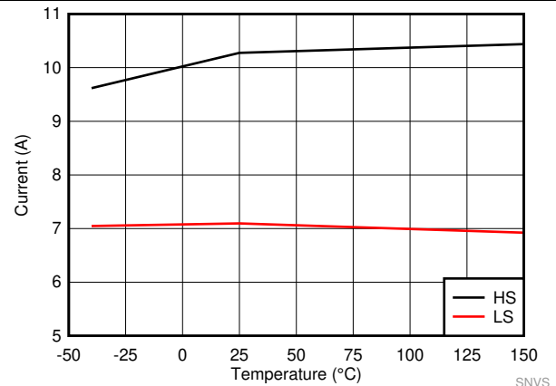
图 4. LM61460 High-side and Low-side Current Limits
