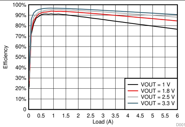
图 1. Efficiency at VIN = PVIN = 5 V
