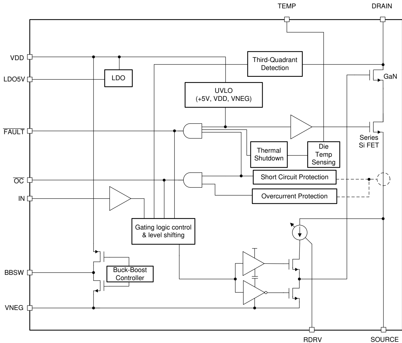
Figure 9-1. Simplified Block Diagram of LMG342xR050
