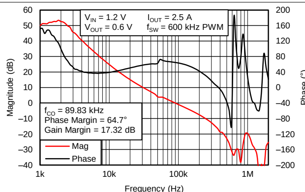
图 34. Bode Plot, Full Load
