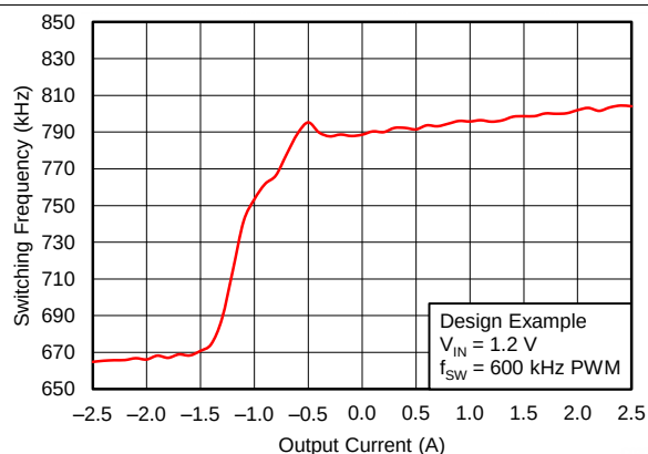
图 35. Switching Frequency vs. Load
