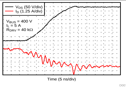
图 6. Turn-off Waveform in Application Example
