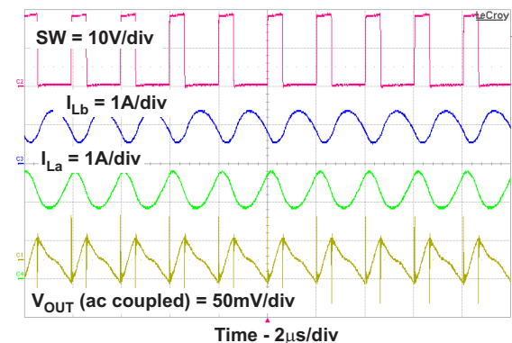
Figure 28. CCM PWM Operation
