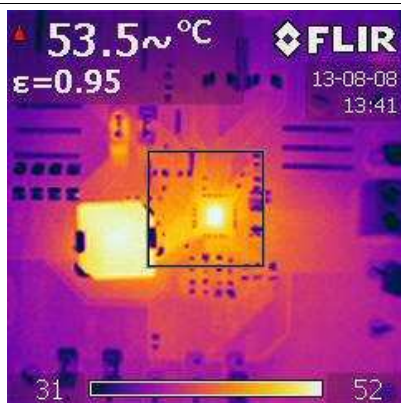
Figure 31. Power Dissipation of TPS55340-EP
