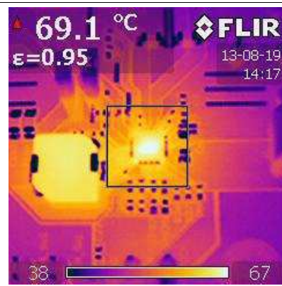
Figure 32. Power Dissipation of TPS55340-EP
