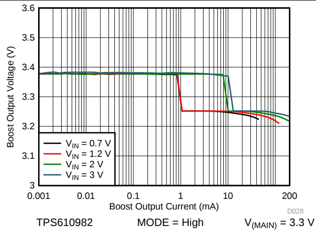
图 25. Boost Load Regulation at Active Mode
