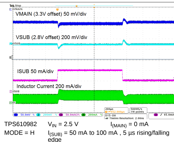
图 73. LDO Load Transient Response
