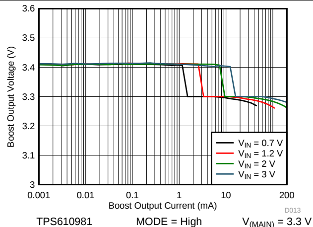
图 23. Boost Load Regulation at Active Mode
