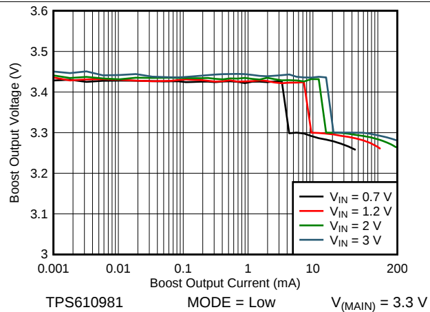
图 22. Boost Load Regulation at Low Power Mode
