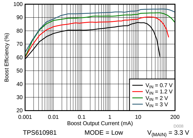
图 16. Boost Efficiency vs Output Current at Low Power Mode
