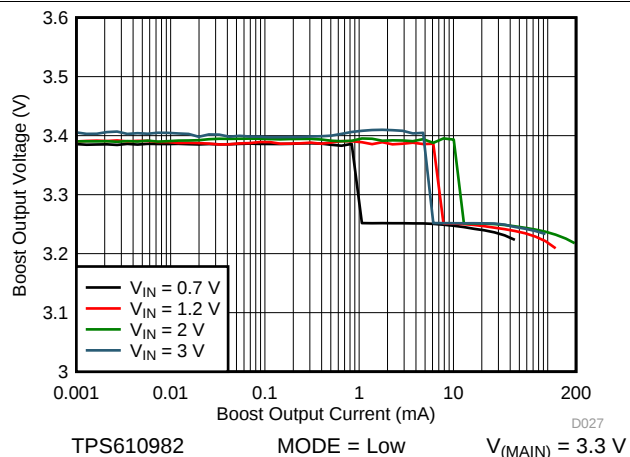
图 24. Boost Load Regulation at Low Power Mode
