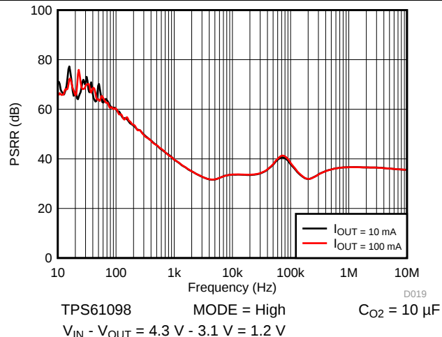
图 35. LDO PSRR vs Frequency
