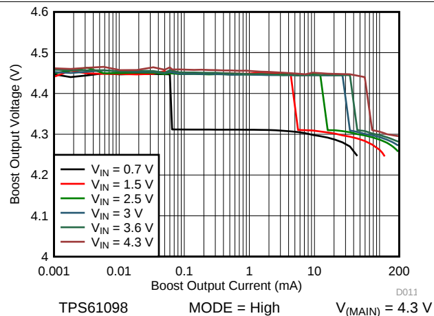
图 21. Boost Load Regulation at Active Mode
