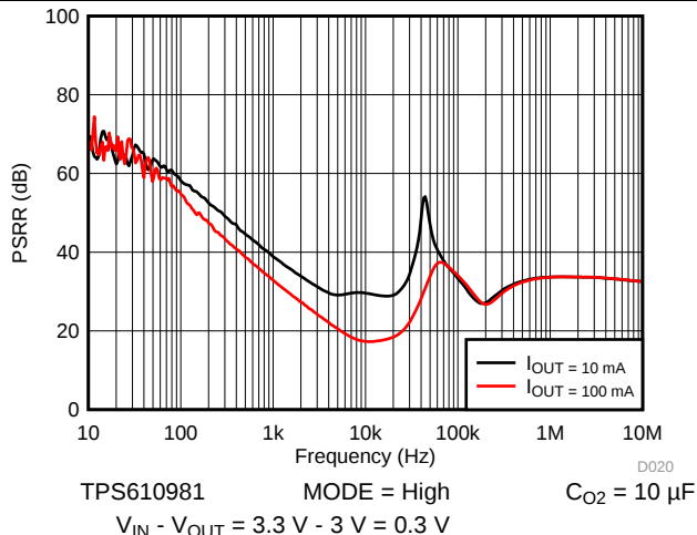
图 36. LDO PSRR vs Frequency
