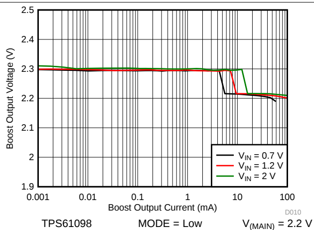
图 20. Boost Load Regulation at Low Power Mode
