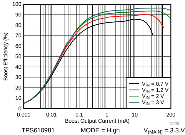
图 17. Boost Efficiency vs Output Current at Active Mode
