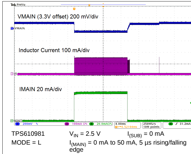
图 51. Load Transient Response
