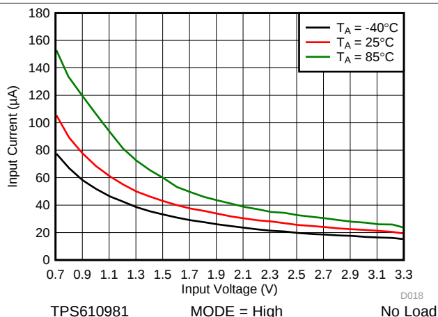
图 32. No Load Input Current vs Input Voltage at Active Mode
