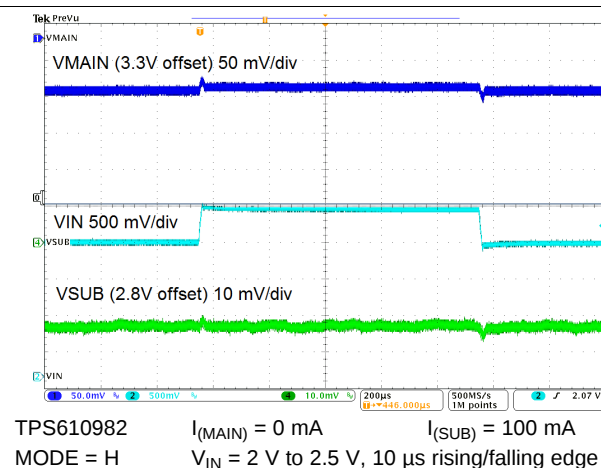
图 71. Line Transient Response
