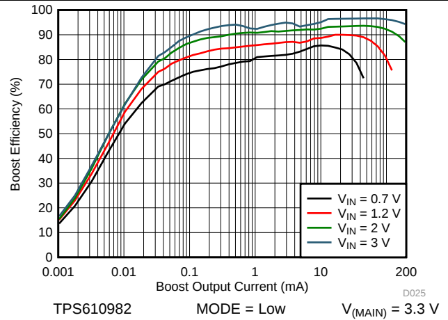
图 18. Boost Efficiency vs Output Current at Low Power Mode
