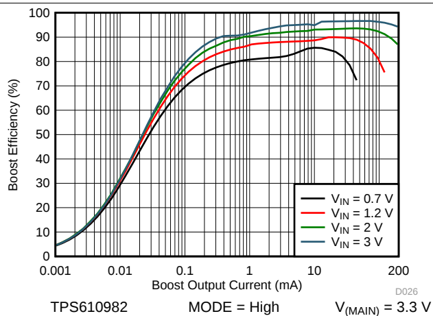
图 19. Boost Efficiency vs Output Current at Active Mode
