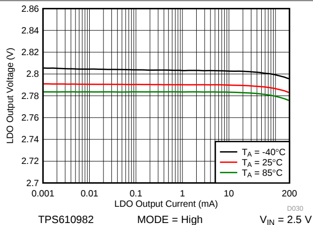
图 29. LDO Load Regulation at Active Mode
