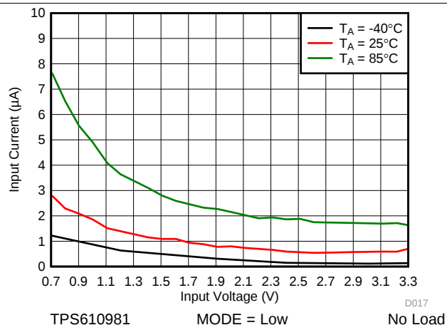
图 31. No Load Input Current vs Input Voltage at Low Power Mode
