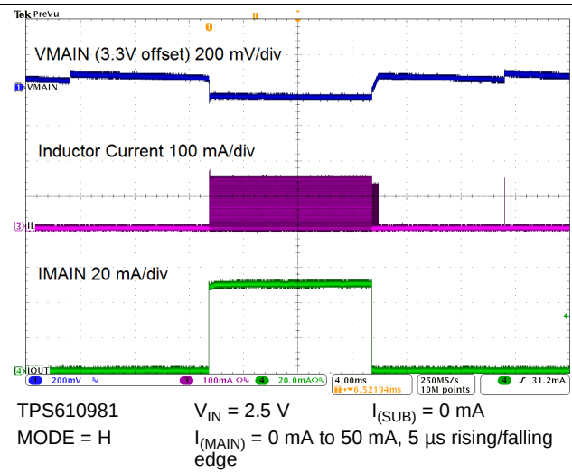
图 52. Load Transient Response
