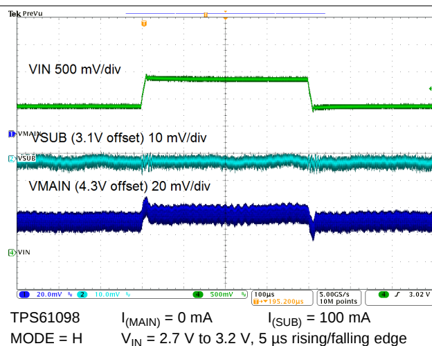
图 69. Line Transient Response
