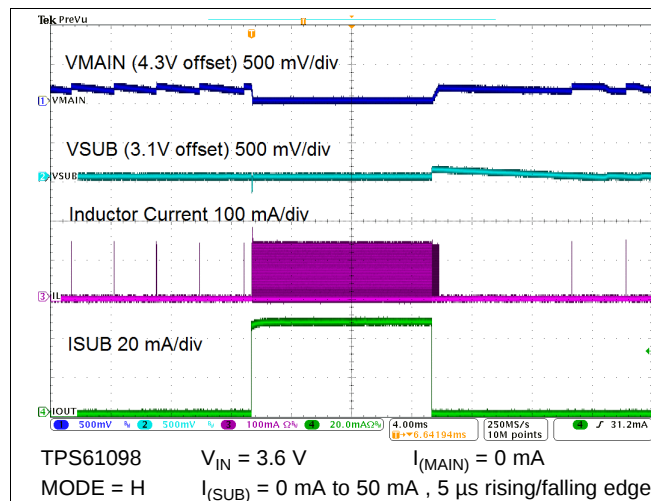
图 68. LDO Load Transient Response
