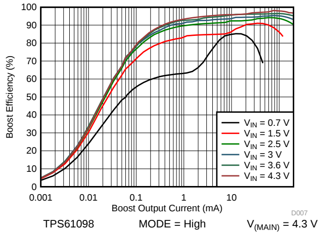
图 15. Boost Efficiency vs Output Current at Active Mode
