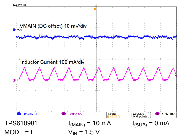
图 46. Switching Waveforms
