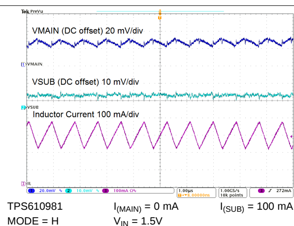
图 50. Switching Waveforms
