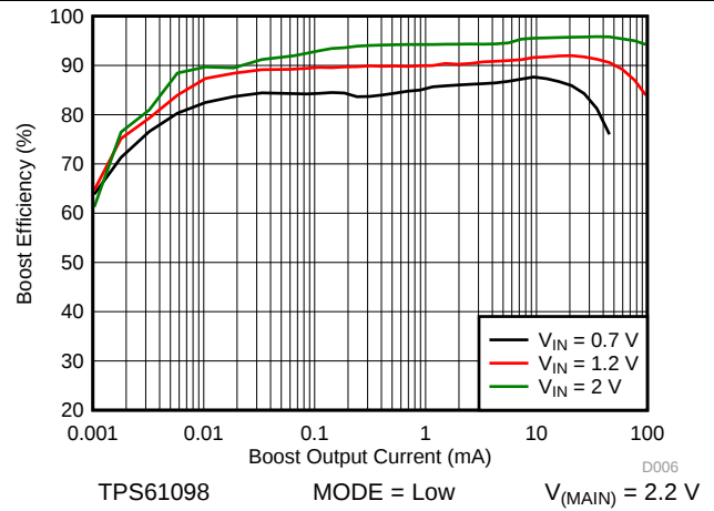
图 14. Boost Efficiency vs Output Current at Low Power Mode
