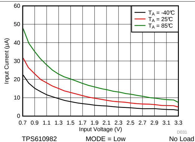
图 33. No Load Input Current vs Input Voltage at Low Power Mode
