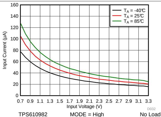
图 34. No Load Input Current vs Input Voltage at Active Mode
