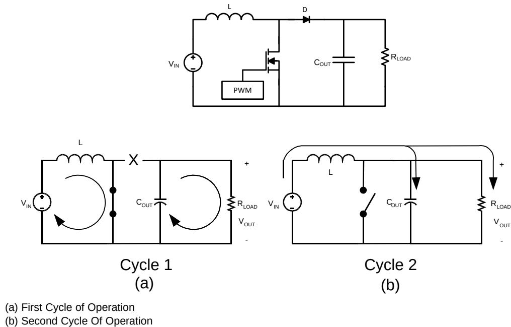
Figure 44. Simplified Boost Converter Diagram
