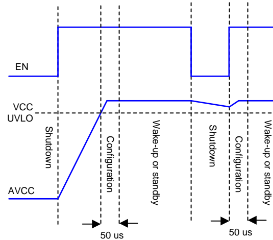
图 9. Power-On Voltage Selection
