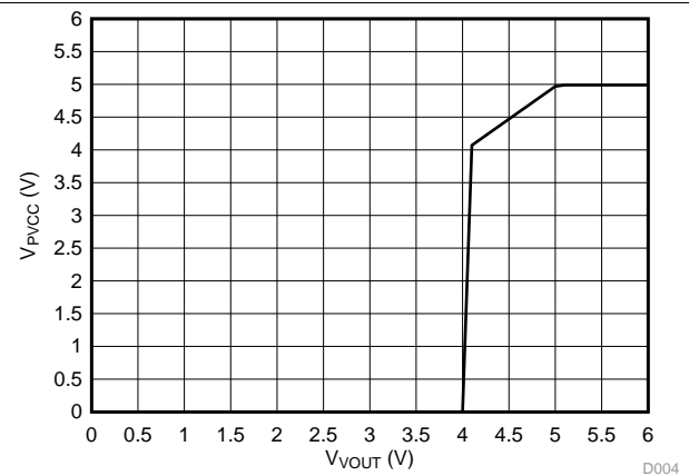
图 4. V_{PVCC} vs V_{VOUT} ( EN = 3.3 \text{ V} , I_{PVCC} = 10 \text{ mA} , V_{OUT} Rising)
