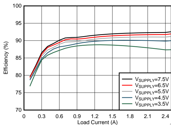
效率 ( V_{LOAD} = 9.5V , F_{SW} = 440kHz )
