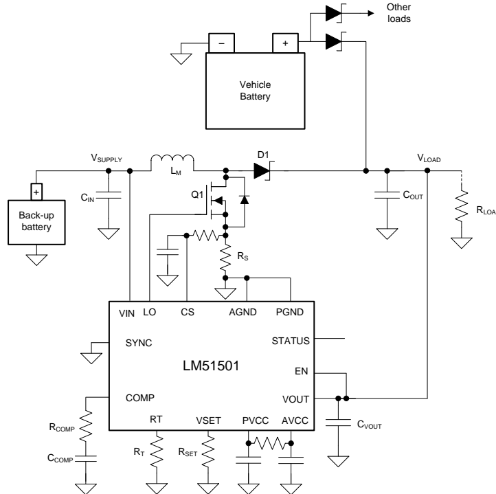
图 16. Typical Emergency Call Application
