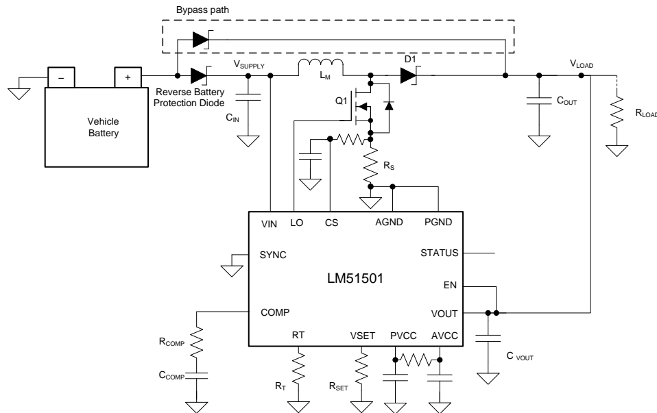
图 15. Typical Start-Stop Application
