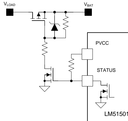
图 18. Disconnection Switch Control Example
