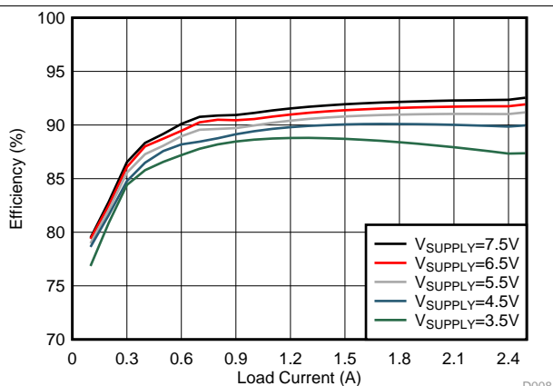
图 8. Efficiency vs Load Current ( V_{LOAD} = 9.5 V , F_{SW} = 440 kHz , SS Configuration)
