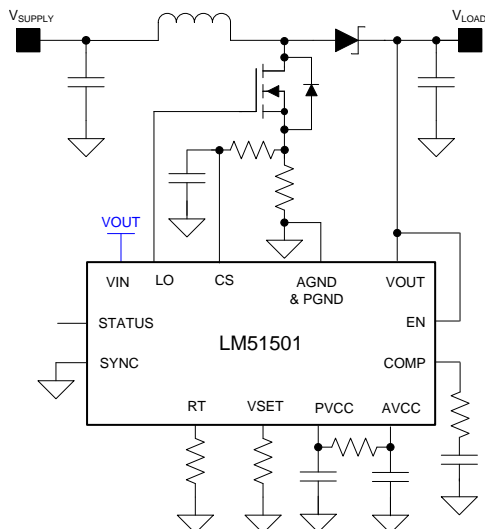
图 22. Lower Standby Threshold in SS Configuration
