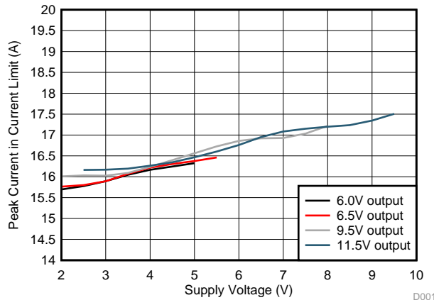
图 1. Peak Inductor Current vs Supply Voltage ( F_{sw} = 440 \text{ kHz} , R_S = 7 \text{ m}\Omega , R_F = 100 \text{ }\Omega , C_F = 2.2 \text{ nF} )
