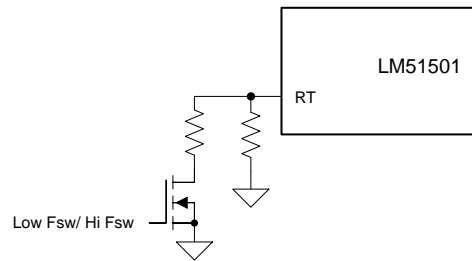
图 25. Dynamic Frequency Change
