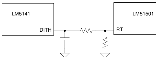
图 23. Dithering Using the Dither-Enabled Device LM5141
