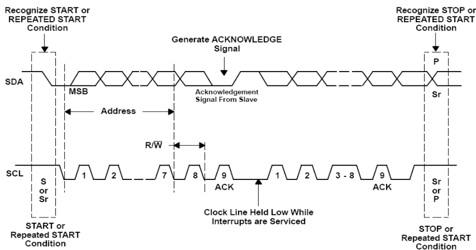
Figure 35. Bus Protocol
