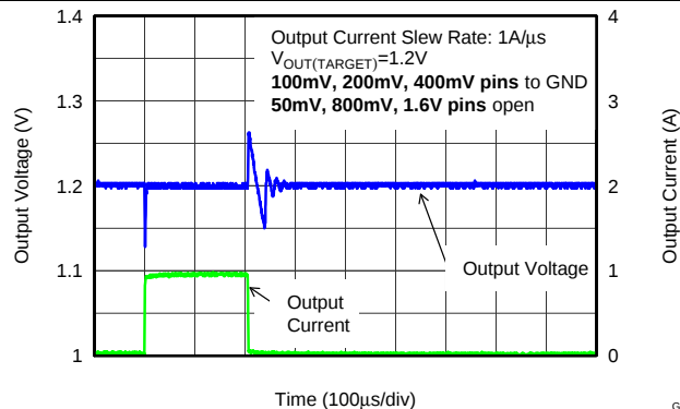
Figure 32. Load Transient Response (V OUT = 1.2 V)
