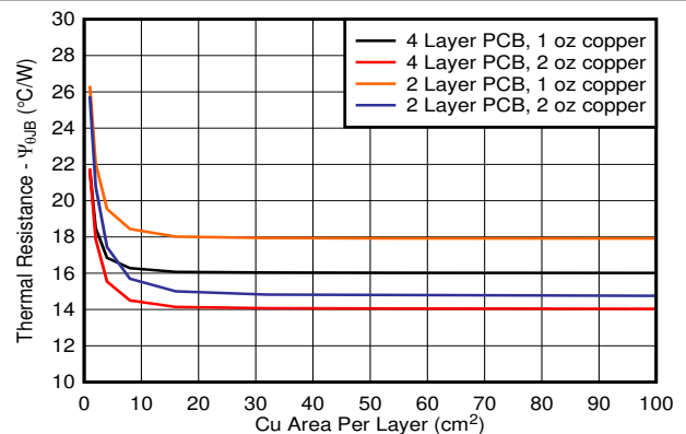
图 8-3. R_{\psi JB} vs Copper Area 2s2p DRC Package
