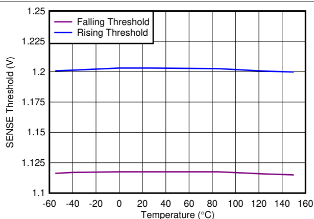
图 6-28. Undervoltage Lockout (UVLO) Threshold vs Temperature
