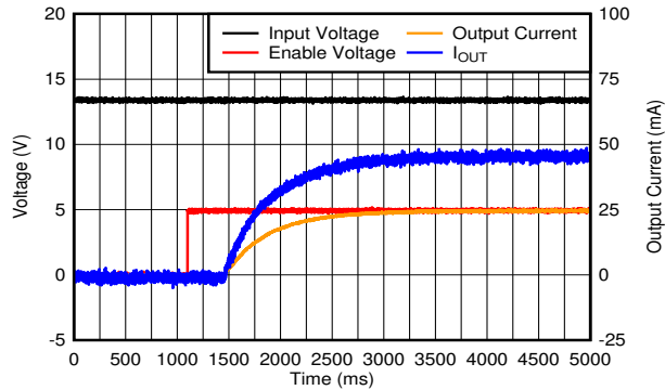
图 8-13. Power-Up Waveform
