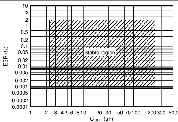
图 6-38. Stability ESR vs C_{OUT}
