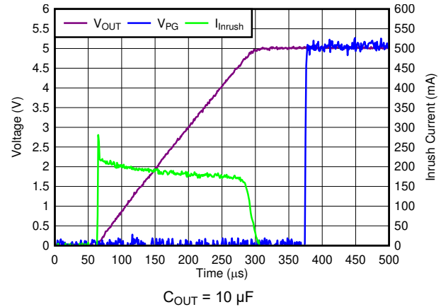
图 6-32. Startup Plot Inrush Current
