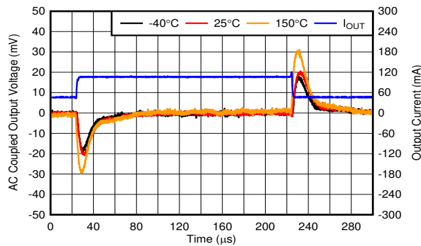
图 8-15. Transient Response
