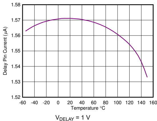
图 6-35. Delay Pin Current vs Temperature
