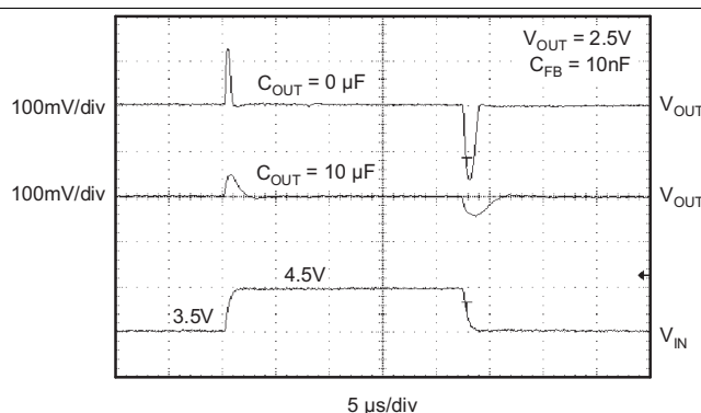
Figure 28. TPS73601 Line Transient, Adjustable Version
