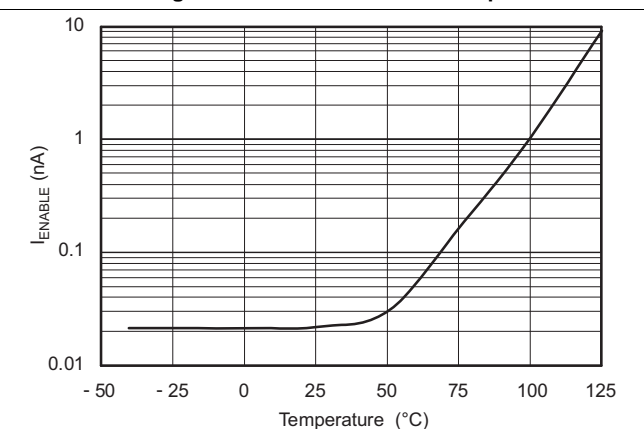
Figure 24. I_{ENABLE} vs Temperature
