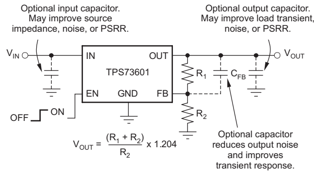
Figure 34. Typical Application Circuit for Adjustable-Voltage Version
