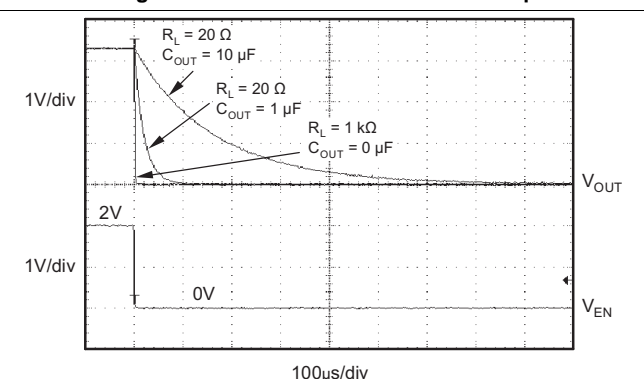
Figure 22. TPS73633 Turnoff Response
