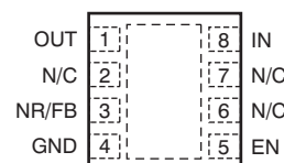
DRB Package 8-Pin VSON Top View
