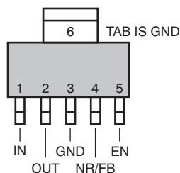
DCQ Package 6-Pin SOT-223 Top View
