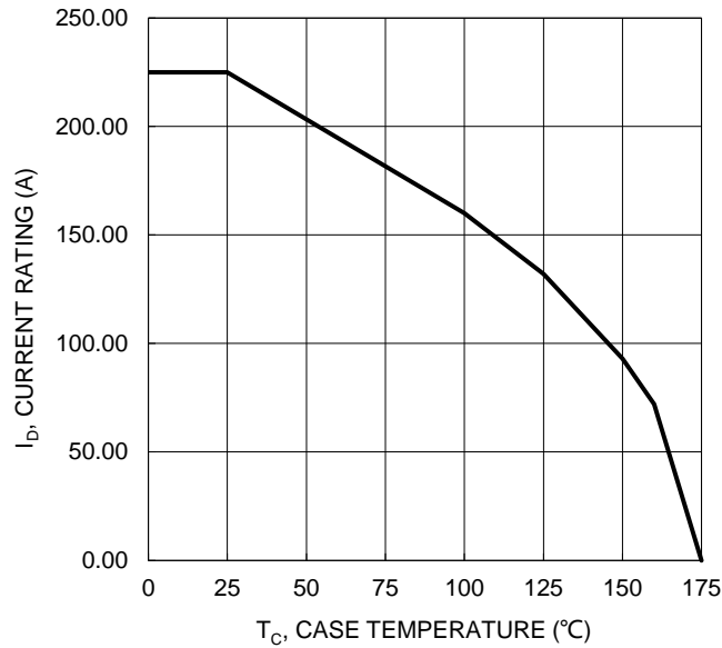
Figure 13. Current Derating
