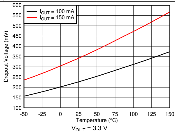
图 7. Dropout Voltage vs Ambient Temperature
