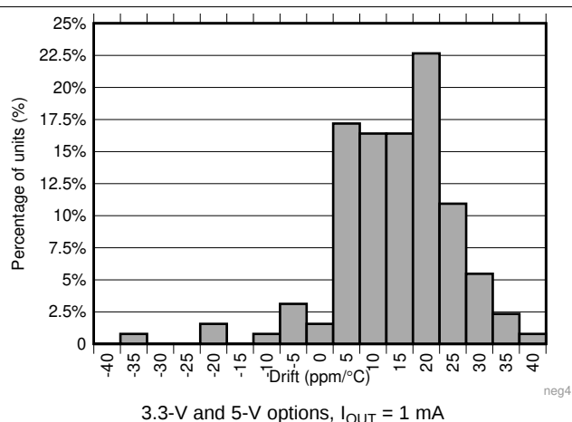
图 10. Temperature Drift Histogram ( -40^{\circ}\text{C} to +25^{\circ}\text{C} )
