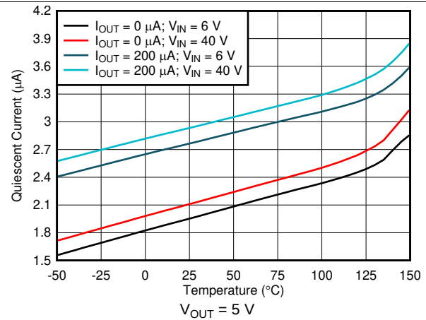
图 2. Quiescent Current vs Ambient Temperature
