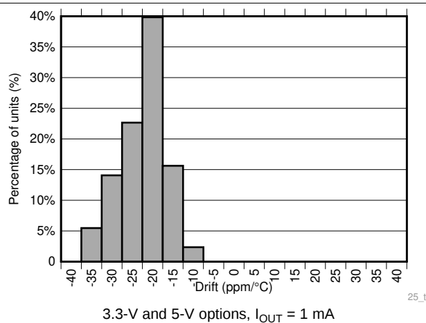
图 11. Temperature Drift Histogram ( 25^{\circ}\text{C} to 150^{\circ}\text{C} )
