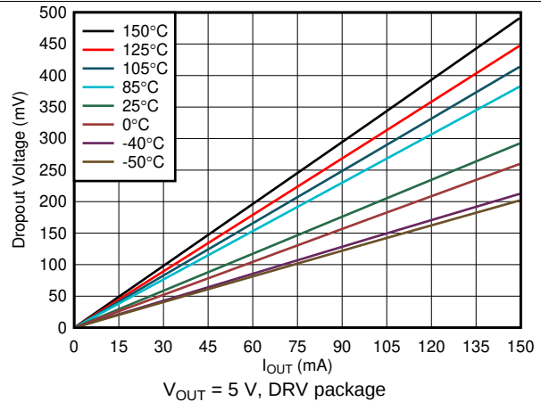
图 4. Dropout Voltage vs Output Current
