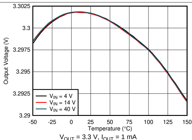
图 9. Output Voltage vs Ambient Temperature
