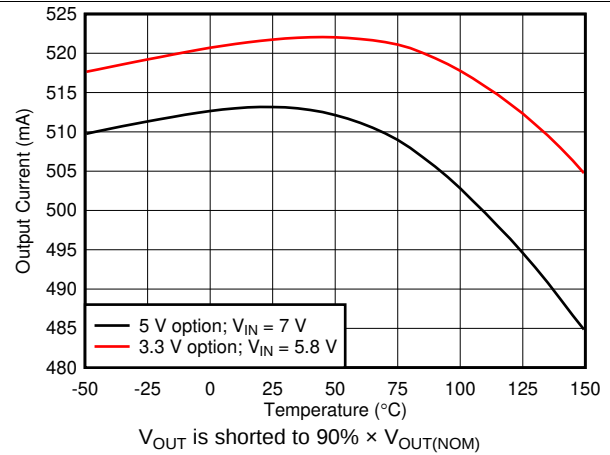
图 14. Output Current Limit vs Ambient Temperature
