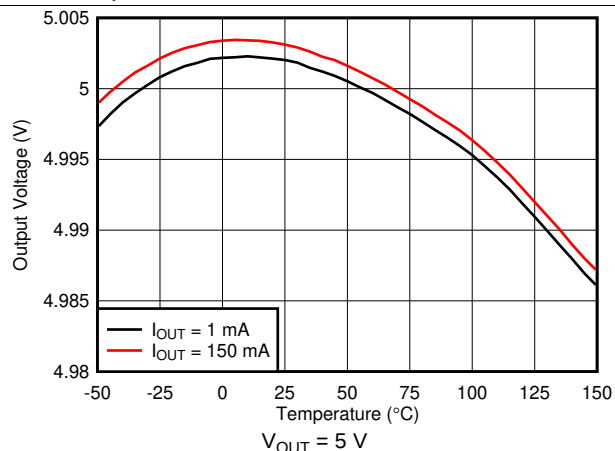
图 8. Output Voltage vs Ambient Temperature
