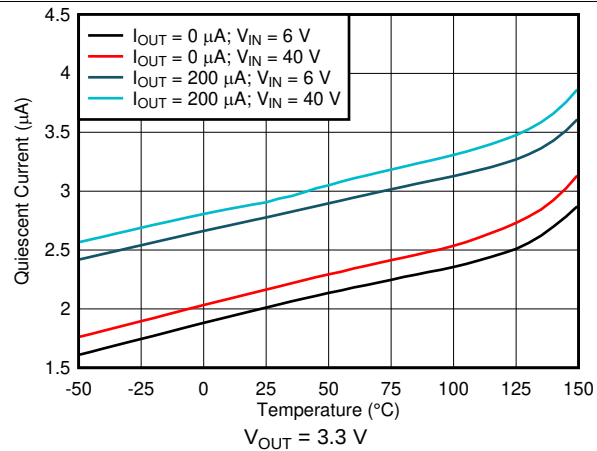
图 3. Quiescent Current vs Ambient Temperature
