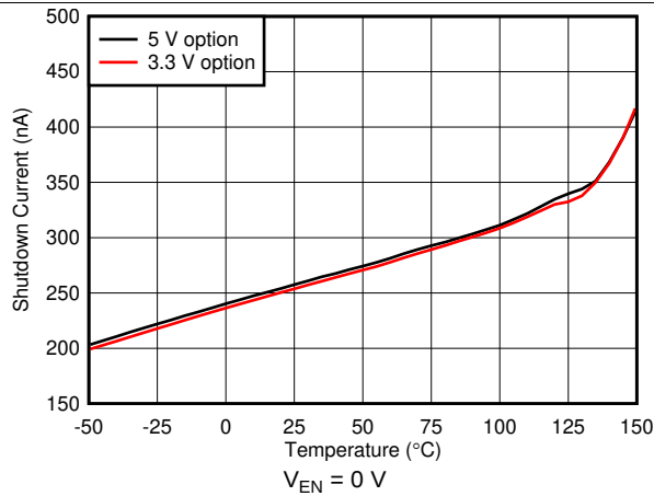
图 1. Shutdown Current vs Ambient Temperature
