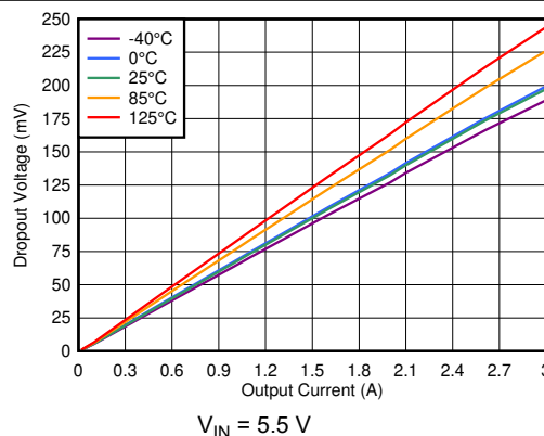
图 6-24. Dropout Voltage vs I_{OUT} (High V_{IN} )
