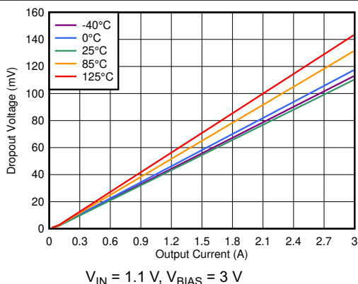
图 6-23. Dropout Voltage vs I_{OUT} With Bias
