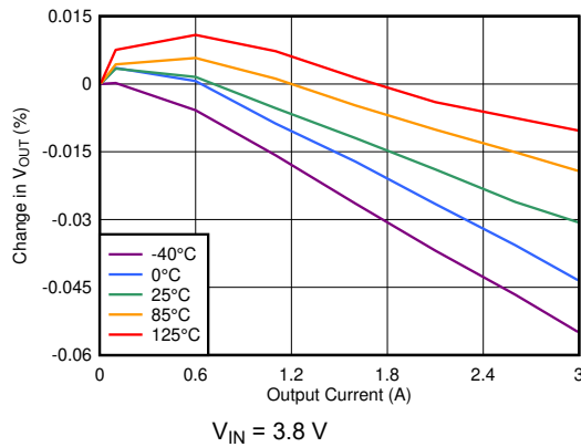
图 6-27. Load Regulation vs I_{OUT} (3.3-V Output)
