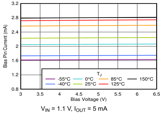
图 6-79. Bias Pin Current With Bias
