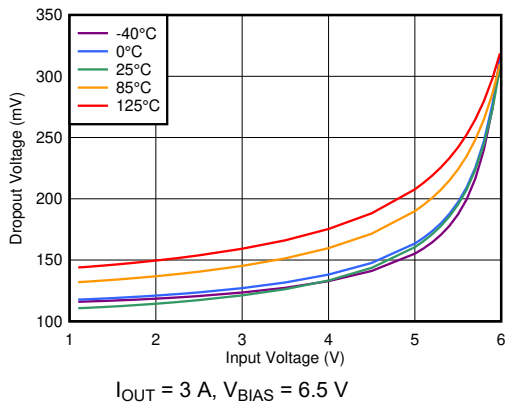
图 6-21. Dropout Voltage vs V_{IN} With Bias
