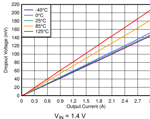
图 6-22. Dropout Voltage vs I_{OUT} Without Bias
