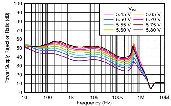
图 6-50. PSRR vs Frequency and V_{IN} ( V_{OUT} = 5\text{ V} )
