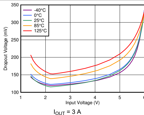
图 6-20. Dropout Voltage vs V_{IN} Without Bias
