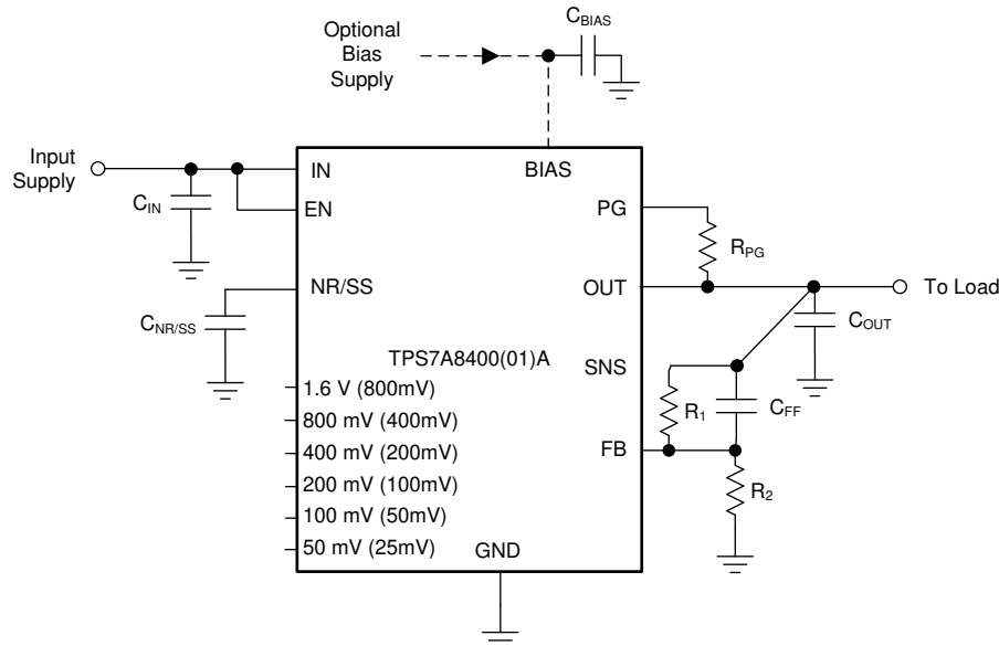
图 8-1. Adjustable Operation
