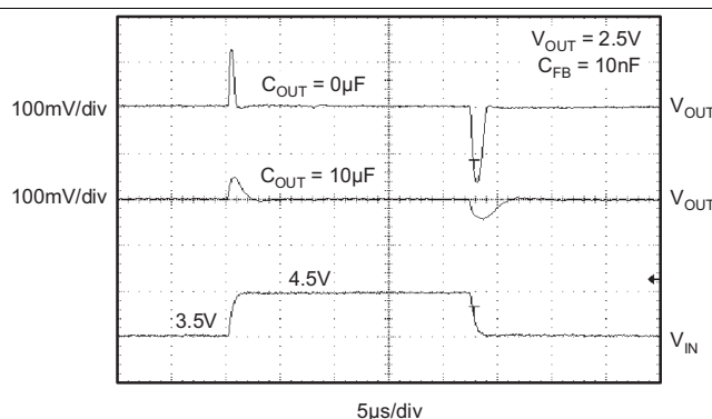
Figure 28. TPS73201-Q1 – Line Transient, Adjustable Version
