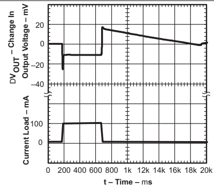
Figure 26. TPS79118 Load Transit Response
