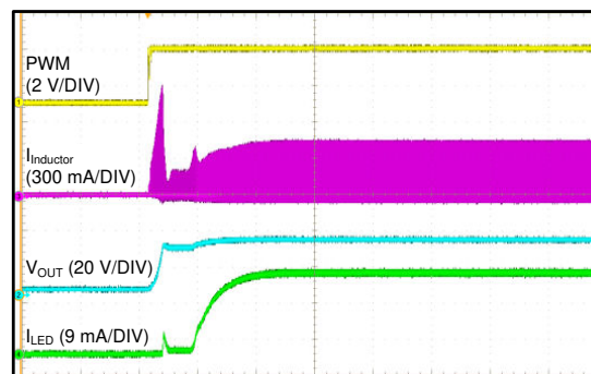
图 8-9. Start-Up Dimming Duty = 100%
